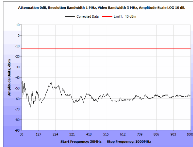
Plot 97. Radiated Spurious Emissions, Low Channel, 30 MHz – 1 GHz, Part 24
