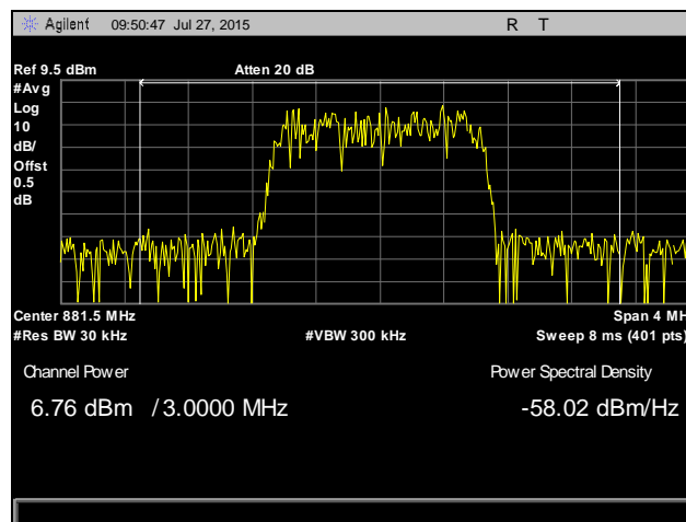
Plot 2. RF Power, Single Channel Operation – High Power, Input CDMA, Mid Channel, Part 22
