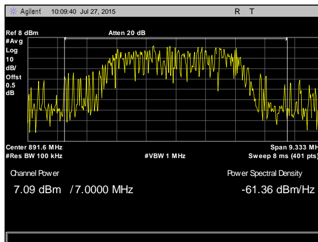
Plot 15. RF Power, Single Channel Operation – High Power, Input WCDMA, High Channel, Part 22
