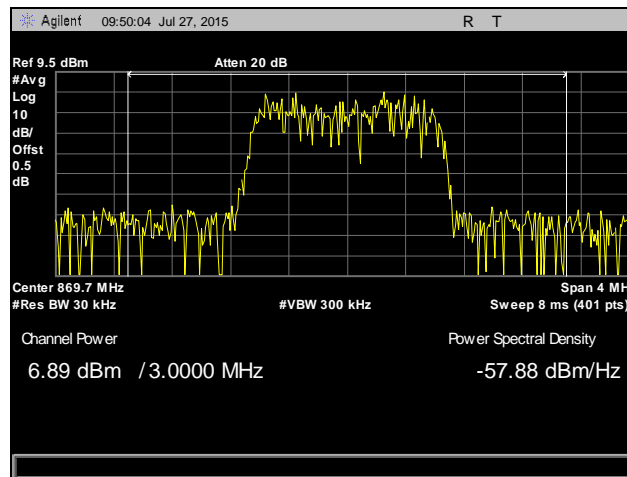
Plot 1. RF Power, Single Channel Operation – High Power, Input CDMA, Low Channel, Part 22
