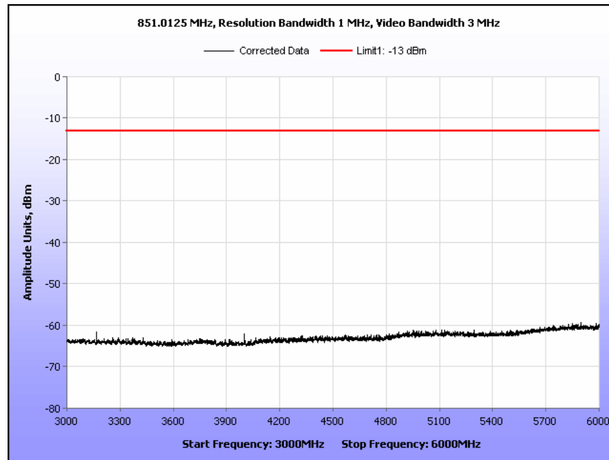
Plot 7. Radiated Spurious Emissions, 851.0125 MHz, 3 GHz – 6 GHz
