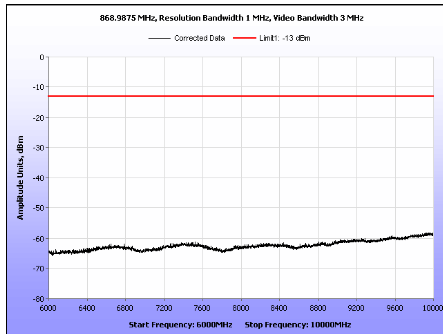
Plot 20. Radiated Spurious Emissions, 868.9875 MHz, 6 GHz – 10 GHz
