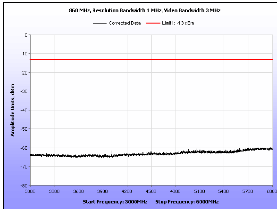
Plot 15. Radiated Spurious Emissions, 860 MHz, 3 GHz – 6 GHz
