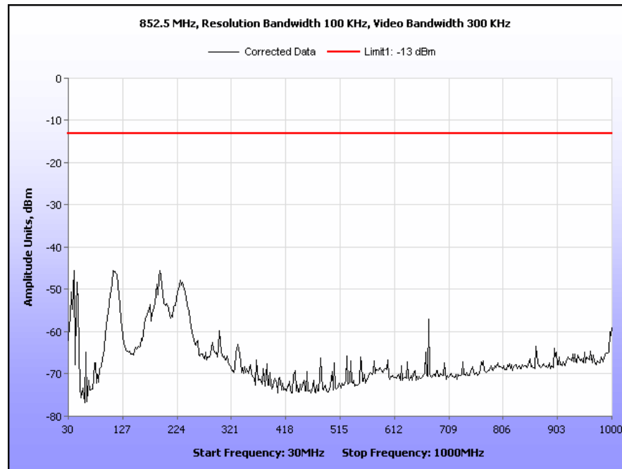
Plot 9. Radiated Spurious Emissions, 852.5 MHz, 30 MHz – 1 GHz
