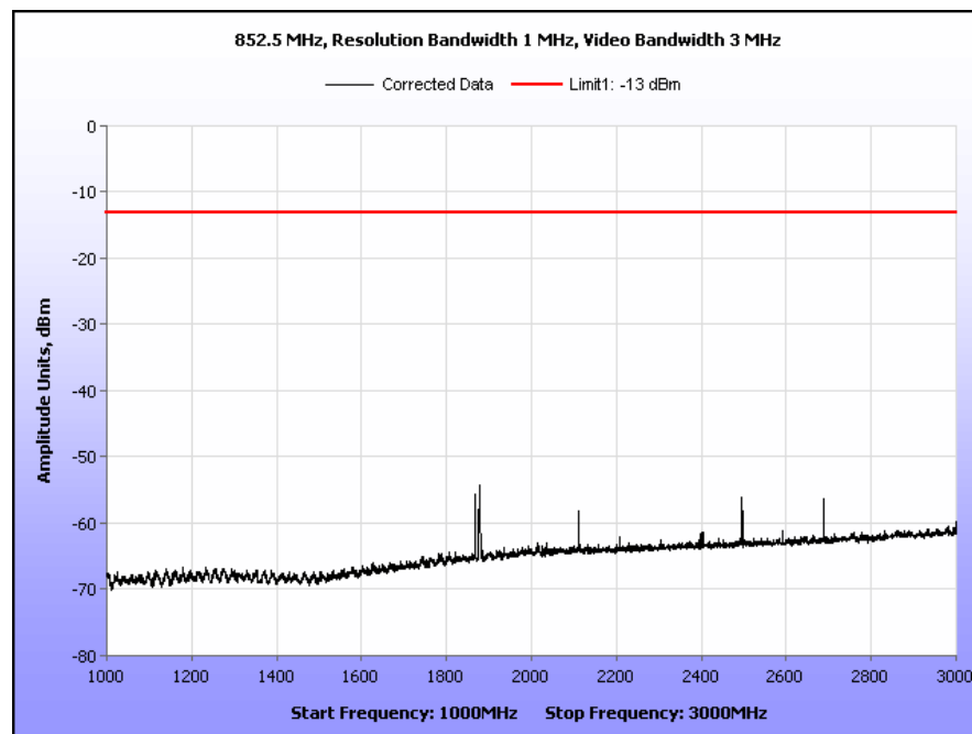
Plot 10. Radiated Spurious Emissions, 852.5 MHz, 1 GHz – 3 GHz
