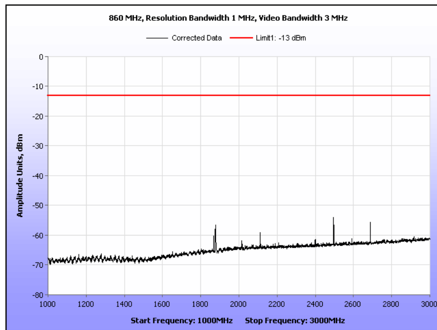
Plot 14. Radiated Spurious Emissions, 860 MHz, 1 GHz – 3 GHz
