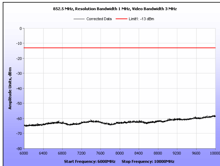
Plot 12. Radiated Spurious Emissions, 852.5 MHz, 6 GHz – 10 GHz
