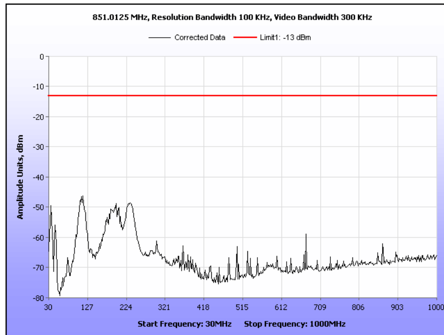
Plot 5. Radiated Spurious Emissions, 851.0125 MHz, 30 MHz – 1 GHz
