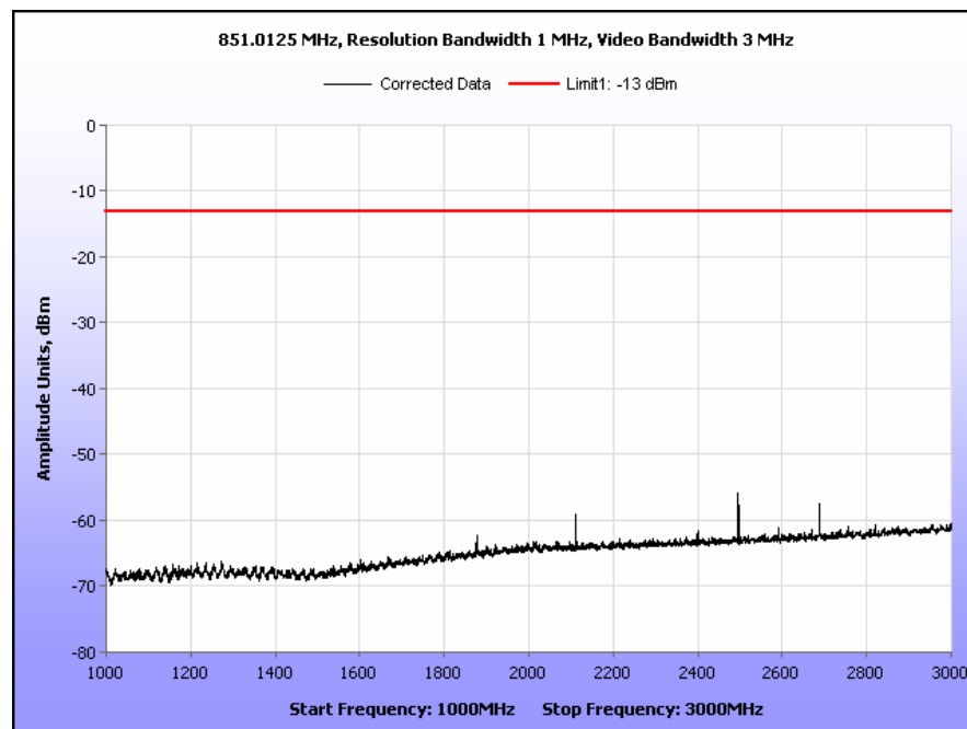
Plot 6. Radiated Spurious Emissions, 851.0125 MHz, 1 GHz – 3 GHz
