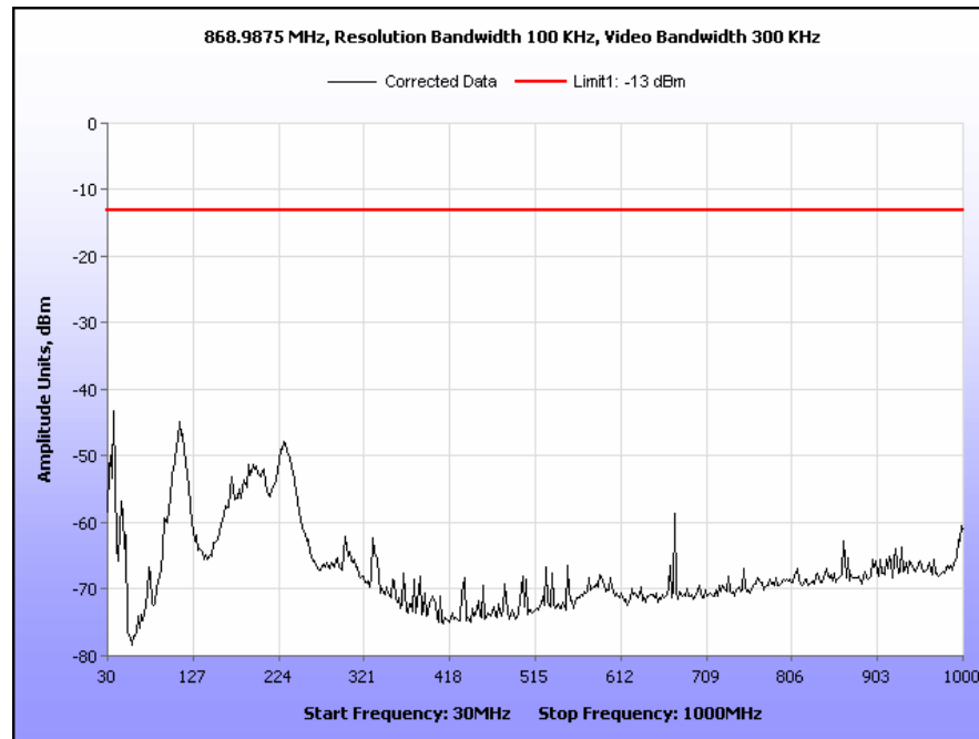
Plot 17. Radiated Spurious Emissions, 868.9875 MHz, 30 MHz – 1 GHz
