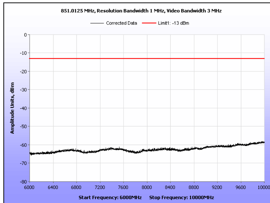
Plot 8. Radiated Spurious Emissions, 851.0125 MHz, 6 GHz – 10 GHz
