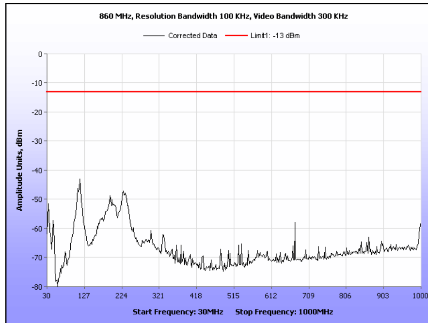
Plot 13. Radiated Spurious Emissions, 860 MHz, 30 MHz – 1 GHz
