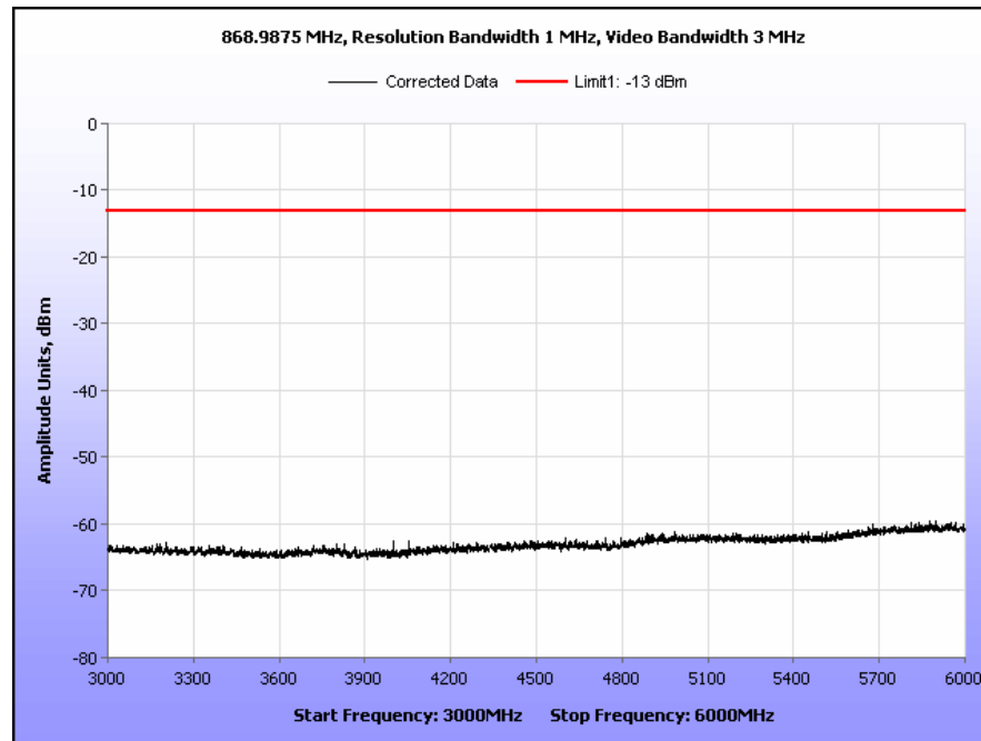
Plot 19. Radiated Spurious Emissions, 868.9875 MHz, 3 GHz – 6 GHz
