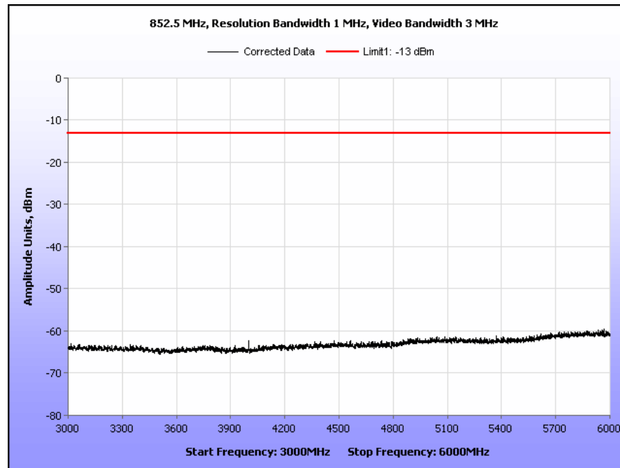
Plot 11. Radiated Spurious Emissions, 852.5 MHz, 3 GHz – 6 GHz
