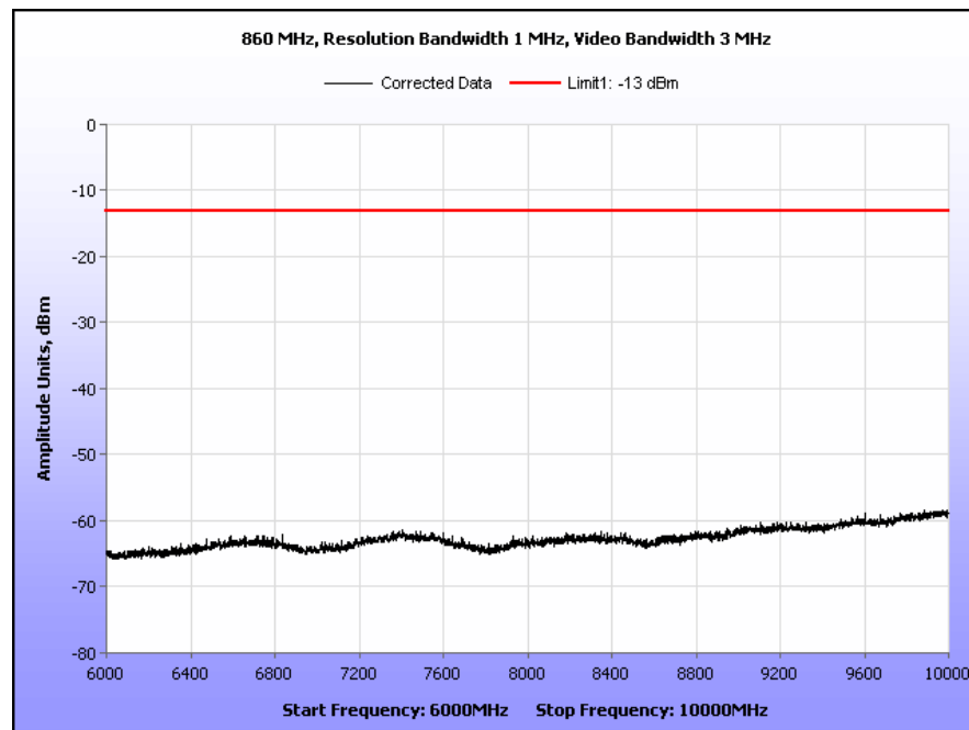
Plot 16. Radiated Spurious Emissions, 860 MHz, 6 GHz – 10 GHz
