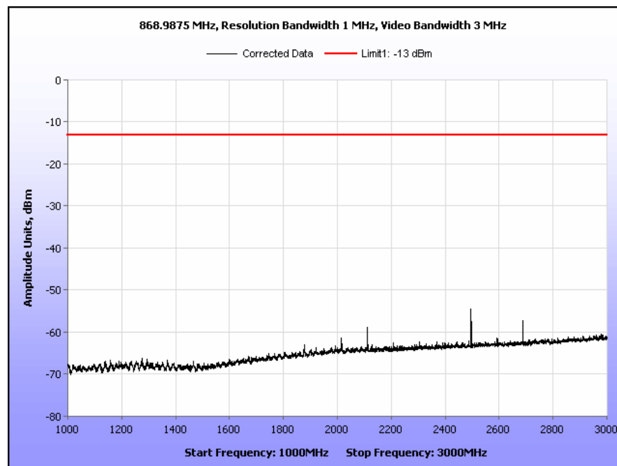
Plot 18. Radiated Spurious Emissions, 868.9875 MHz, 1 GHz – 3 GHz
