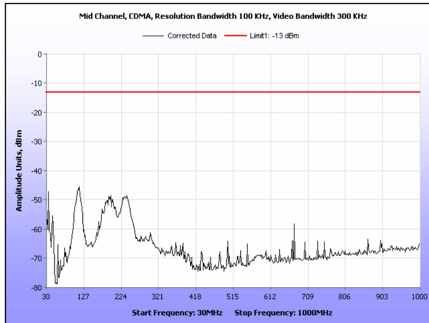
Plot 57. Radiated Spurious Emissions, Mid Channel, CDMA, Part 24, 30 MHz – 1 GHz
