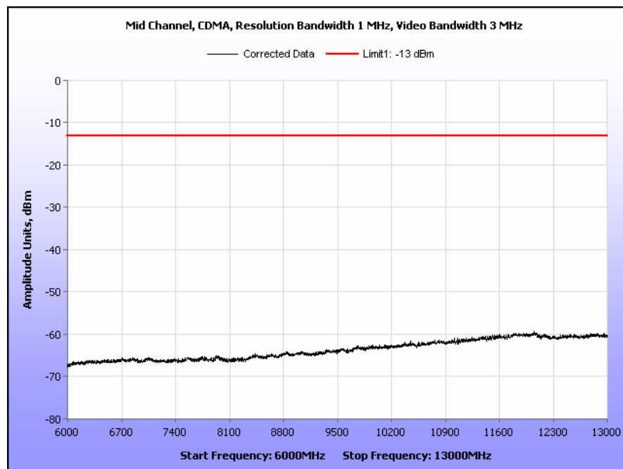
Plot 60. Radiated Spurious Emissions, Mid Channel, CDMA, Part 24, 6 GHz – 13 GHz
