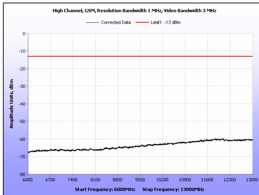
Plot 50. Radiated Spurious Emissions, High Channel, GSM, Part 24, 6 GHz – 13 GHz
