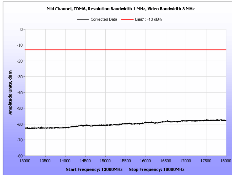
Plot 61. Radiated Spurious Emissions, Mid Channel, CDMA, Part 24, 13 GHz – 18 GHz
