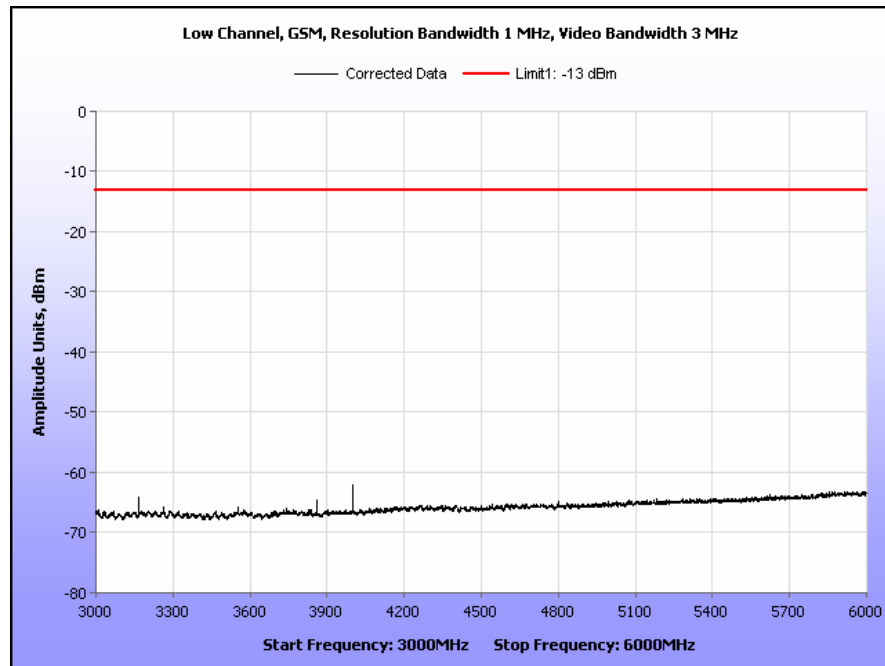
Plot 39. Radiated Spurious Emissions, Low Channel, GSM, Part 24, 3 GHz – 6 GHz
