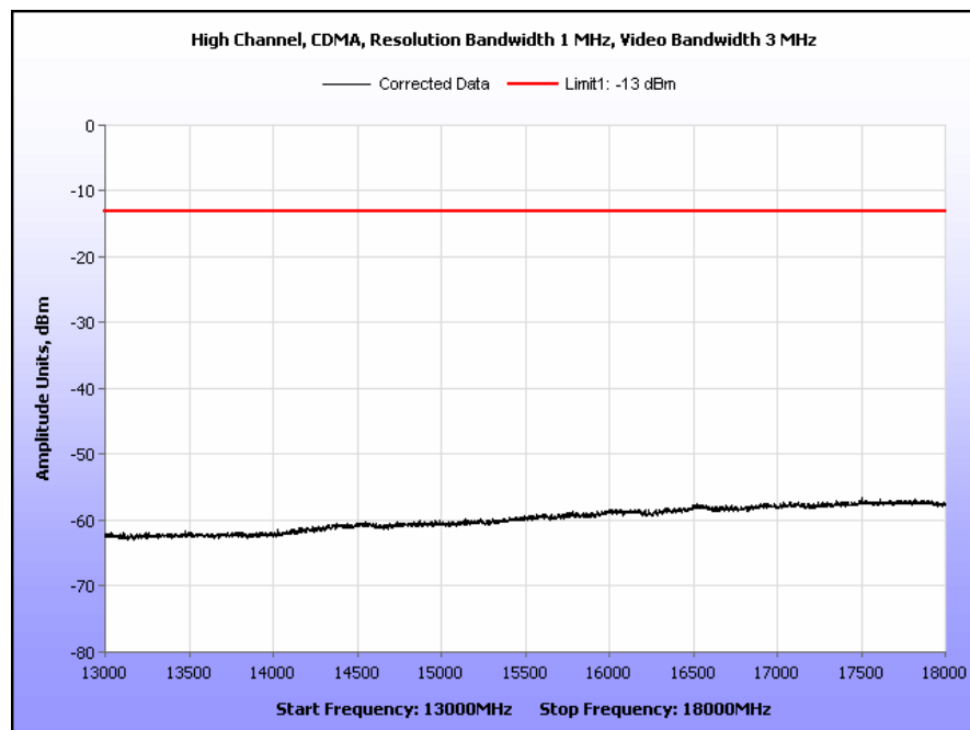
Plot 66. Radiated Spurious Emissions, High Channel, CDMA, Part 24, 13 GHz – 18 GHz
