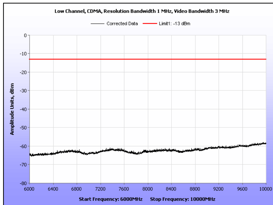
Plot 28. Radiated Spurious Emissions, Low Channel, CDMA, Part 22, 6 GHz – 10 GHz
