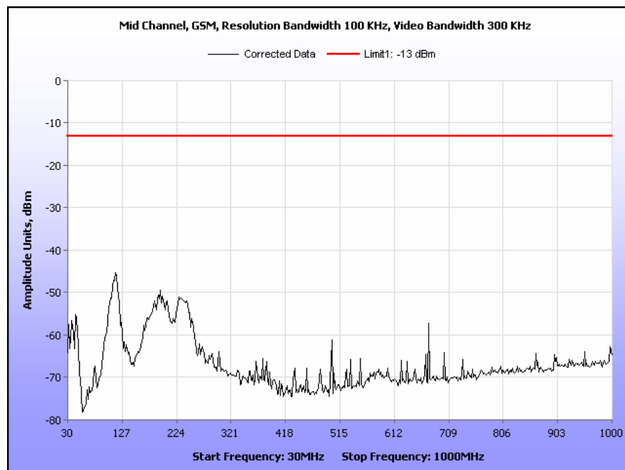
Plot 42. Radiated Spurious Emissions, Mid Channel, GSM, Part 24, 30 MHz – 1 GHz
