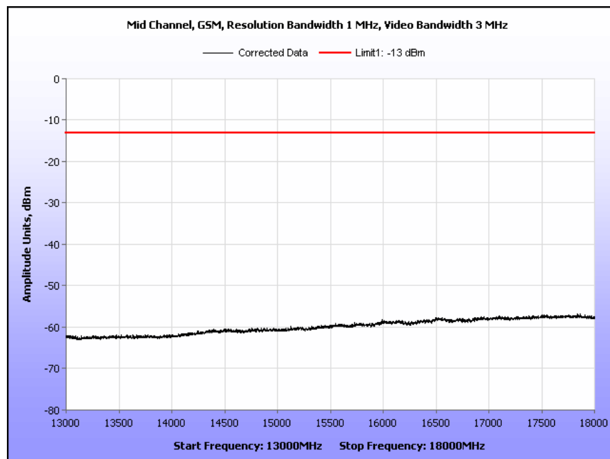
Plot 46. Radiated Spurious Emissions, Mid Channel, GSM, Part 24, 13 GHz – 18 GHz
