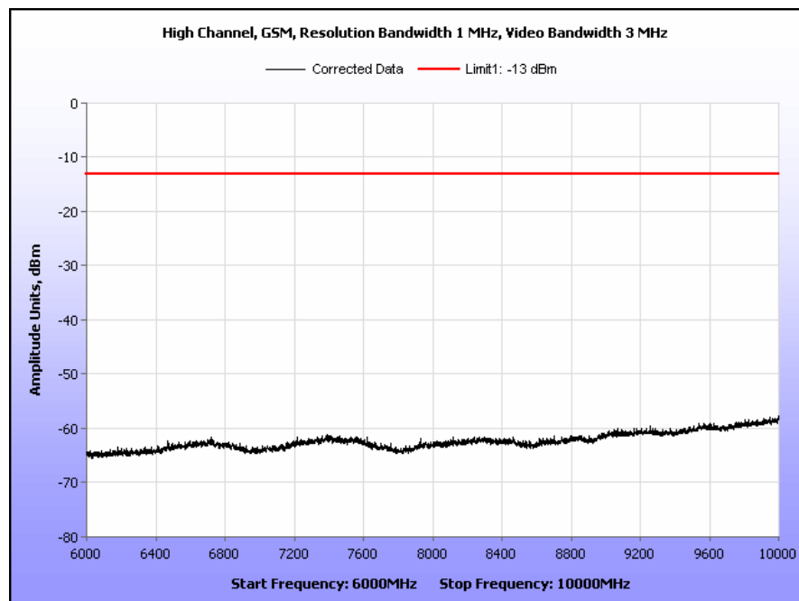
Plot 24. Radiated Spurious Emissions, High Channel, GSM, Part 22, 6 GHz – 10 GHz
