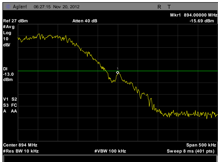
Plot 68. Band Edge, Part 22, GSM, High Channel
