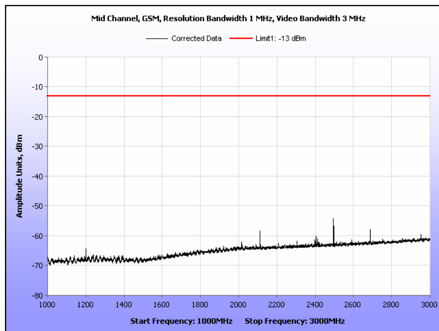
Plot 18. Radiated Spurious Emissions, Mid Channel, GSM, Part 22, 1 GHz – 3 GHz
