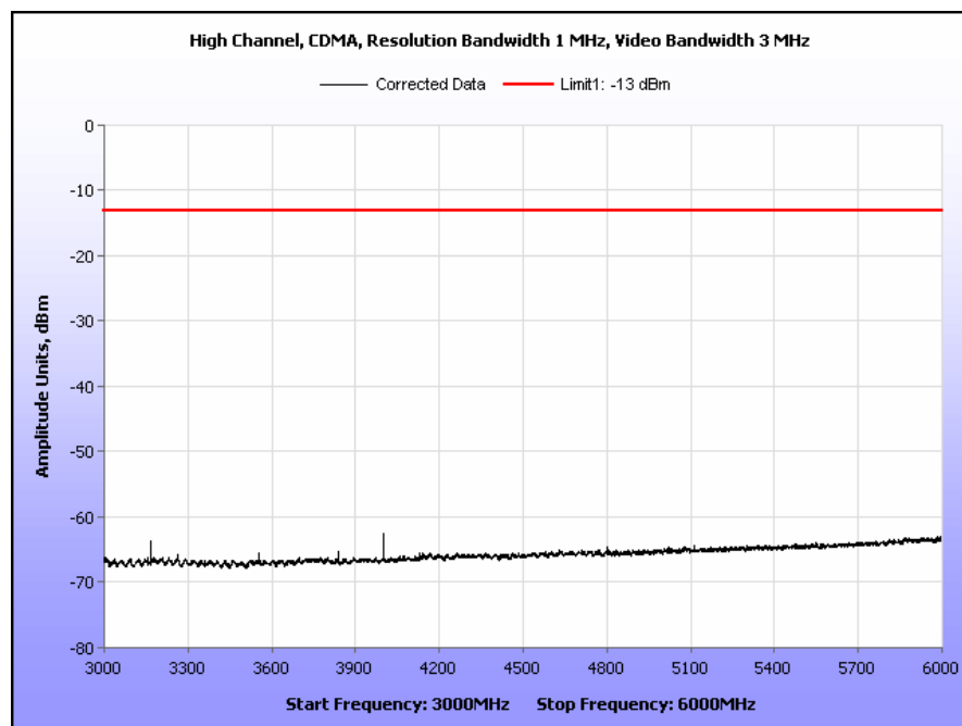
Plot 64. Radiated Spurious Emissions, High Channel, CDMA, Part 24, 3 GHz – 6 GHz
