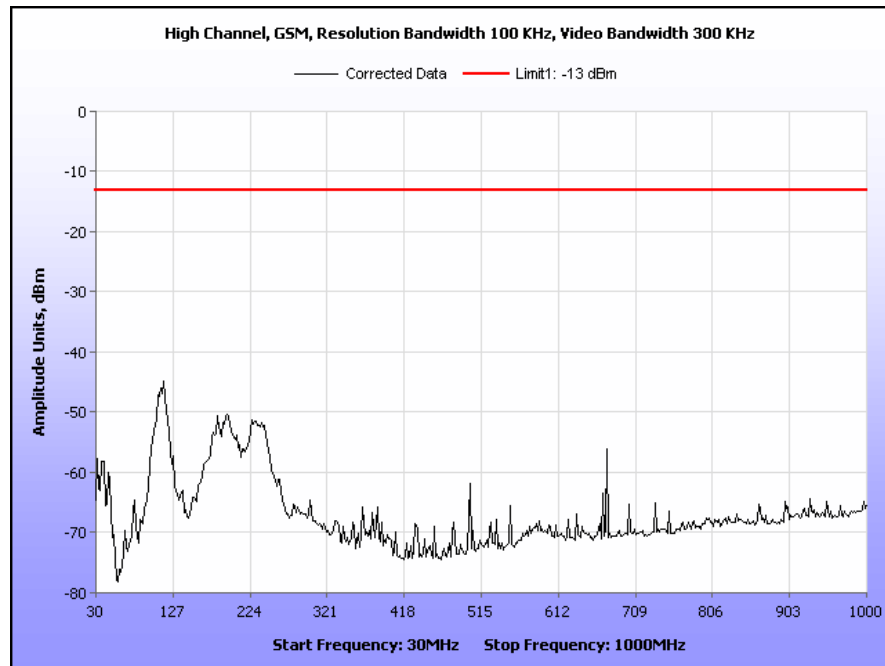
Plot 47. Radiated Spurious Emissions, High Channel, GSM, Part 24, 30 MHz – 1 GHz
