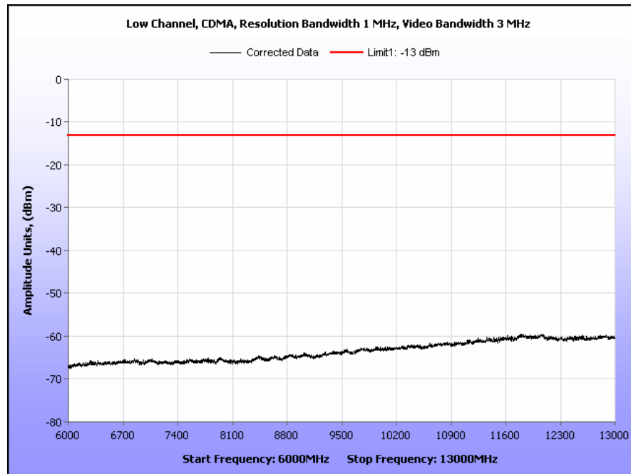
Plot 55. Radiated Spurious Emissions, Low Channel, CDMA, Part 24, 6 GHz – 13 GHz
