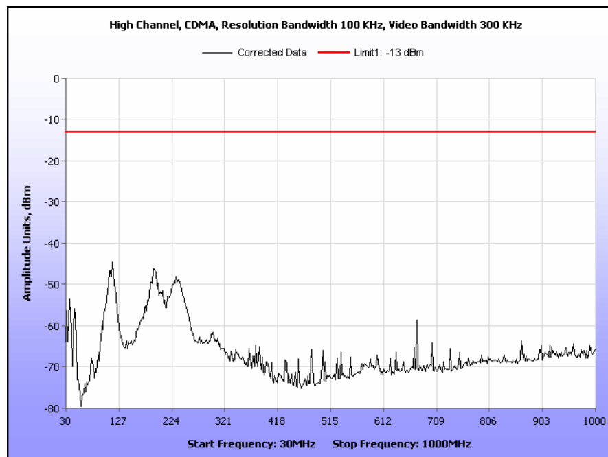
Plot 62. Radiated Spurious Emissions, High Channel, CDMA, Part 24, 30 MHz – 1 GHz
