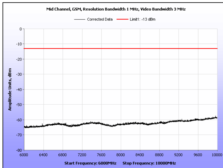
Plot 20. Radiated Spurious Emissions, Mid Channel, GSM, Part 22, 6 GHz – 10 GHz
