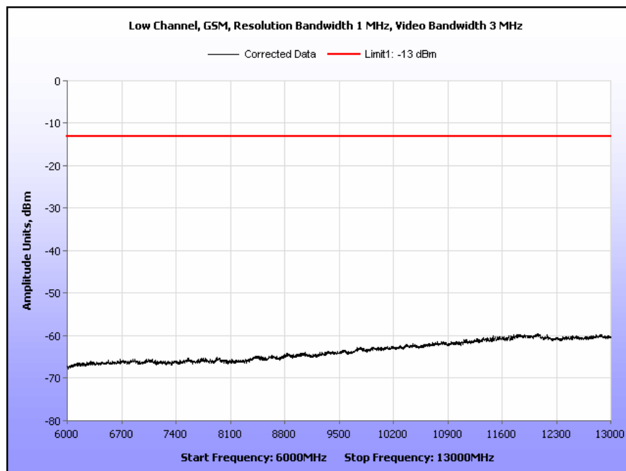
Plot 40. Radiated Spurious Emissions, Low Channel, GSM, Part 24, 6 GHz – 13 GHz
