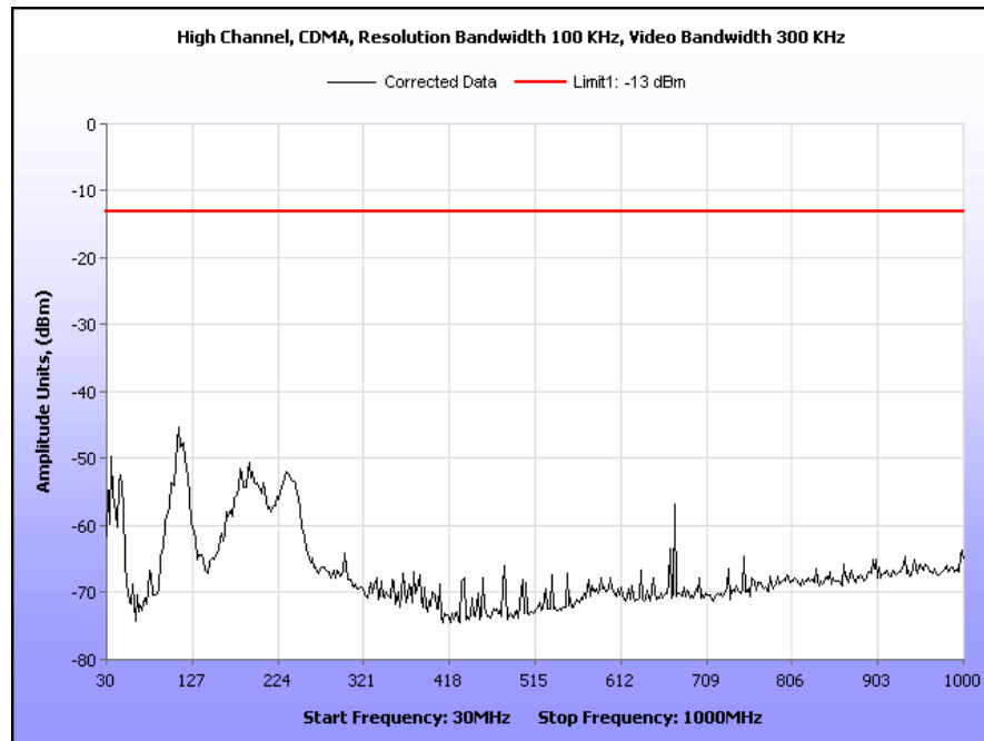
Plot 33. Radiated Spurious Emissions, High Channel, CDMA, Part 22, 30 MHz – 1 GHz
