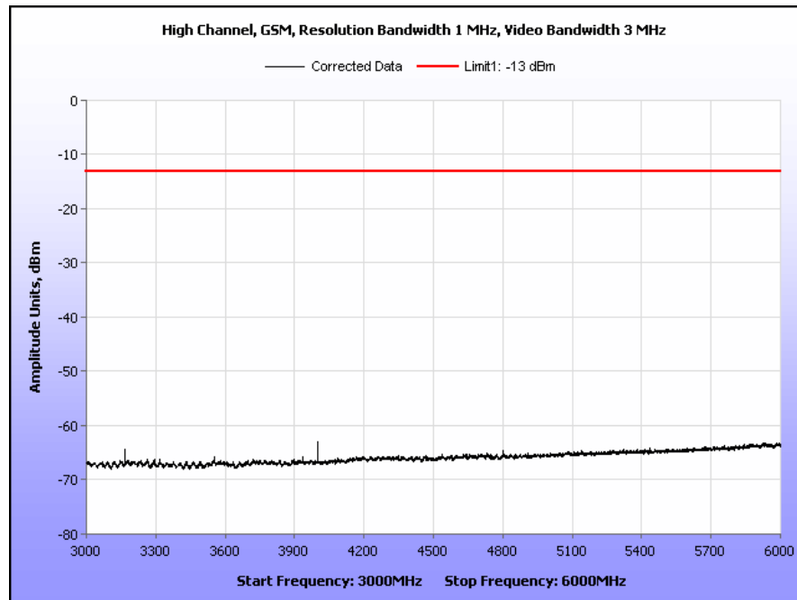
Plot 49. Radiated Spurious Emissions, High Channel, GSM, Part 24, 3 GHz – 6 GHz
