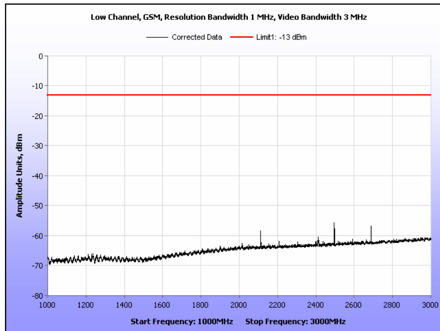
Plot 14. Radiated Spurious Emissions, Low Channel, GSM, Part 22, 1 GHz – 3 GHz
