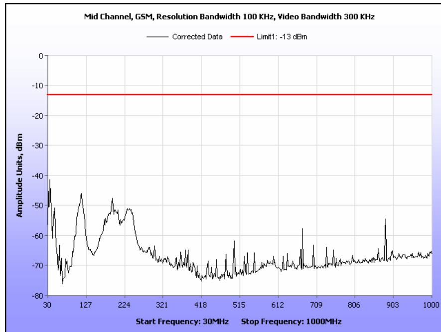
Plot 17. Radiated Spurious Emissions, Mid Channel, GSM, Part 22, 30 MHz – 1 GHz
