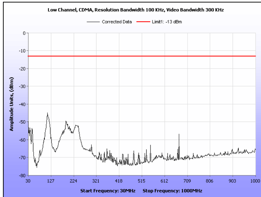
Plot 25. Radiated Spurious Emissions, Low Channel, CDMA, Part 22, 30 MHz – 1 GHz
