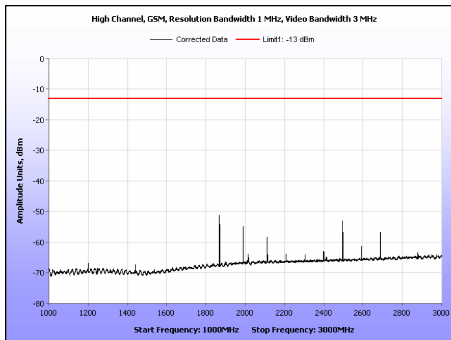
Plot 48. Radiated Spurious Emissions, High Channel, GSM, Part 24, 1 GHz – 3 GHz
