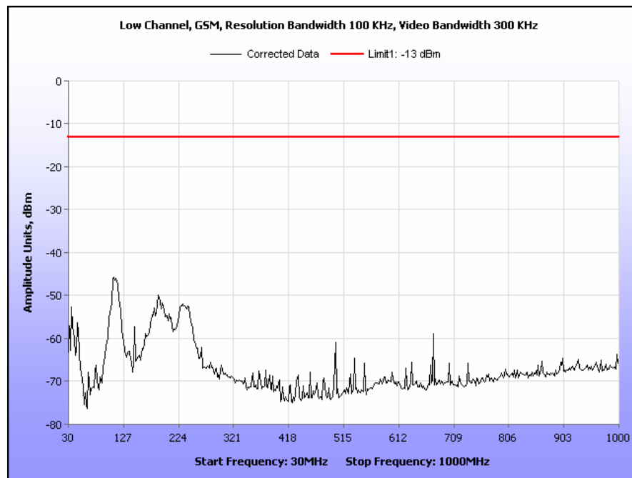
Plot 37. Radiated Spurious Emissions, Low Channel, GSM, Part 24, 30 MHz – 1 GHz
