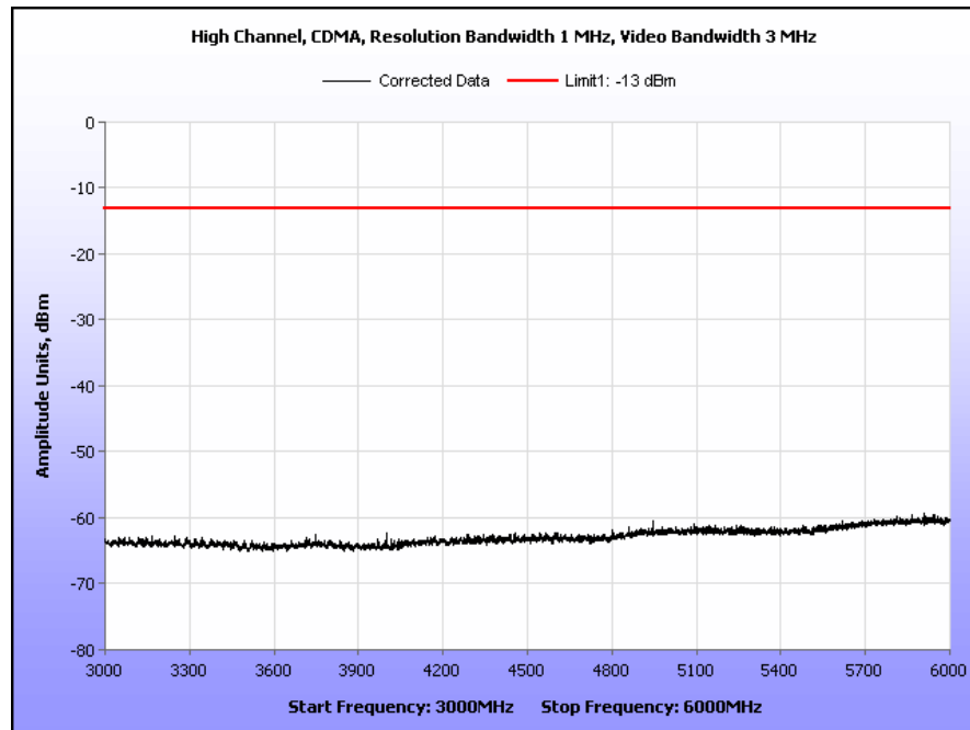
Plot 35. Radiated Spurious Emissions, High Channel, CDMA, Part 22, 3 GHz – 6 GHz
