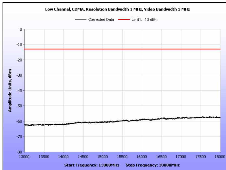
Plot 56. Radiated Spurious Emissions, Low Channel, CDMA, Part 24, 13 GHz – 18 GHz
