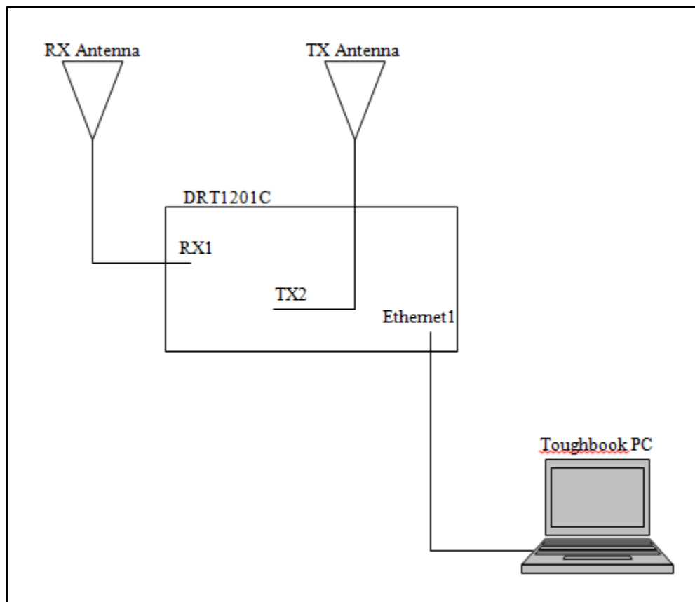
Figure 1. Block Diagram of Equipment Configuration
