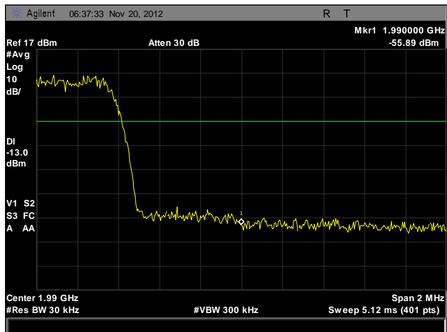
Plot 74. Band Edge, Part 24, CDMA, High Channel
