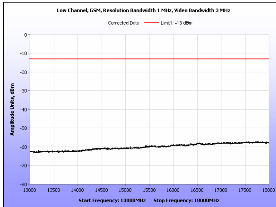
Plot 41. Radiated Spurious Emissions, Low Channel, GSM, Part 24, 13 GHz – 18 GHz
