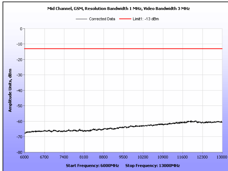
Plot 45. Radiated Spurious Emissions, Mid Channel, GSM, Part 24, 6 GHz – 13 GHz
