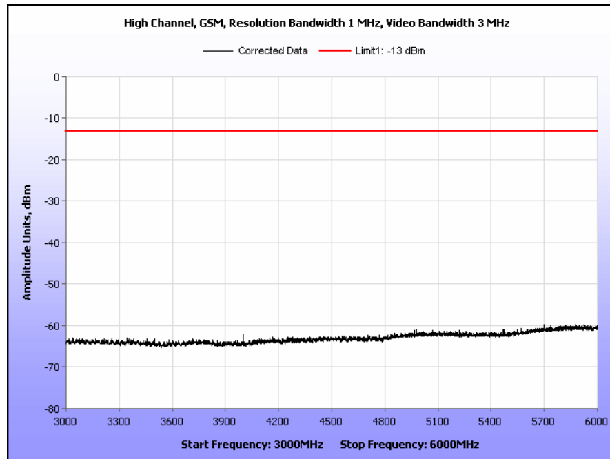
Plot 23. Radiated Spurious Emissions, High Channel, GSM, Part 22, 3 GHz – 6 GHz
