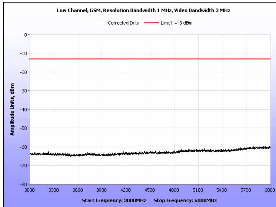
Plot 15. Radiated Spurious Emissions, Low Channel, GSM, Part 22, 3 GHz – 6 GHz
