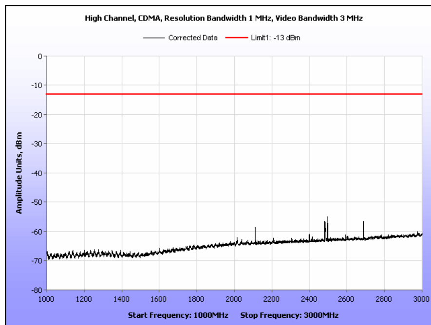
Plot 34. Radiated Spurious Emissions, High Channel, CDMA, Part 22, 1 GHz – 3 GHz
