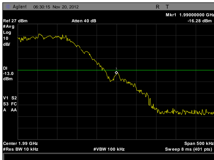
Plot 72. Band Edge, Part 24, GSM, High Channel
