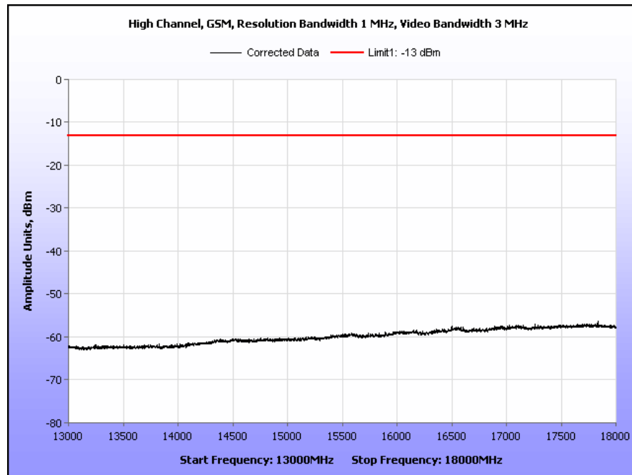
Plot 51. Radiated Spurious Emissions, High Channel, GSM, Part 24, 13 GHz – 18 GHz
