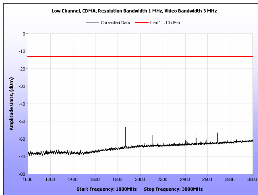
Plot 26. Radiated Spurious Emissions, Low Channel, CDMA, Part 22, 1 GHz – 3 GHz
