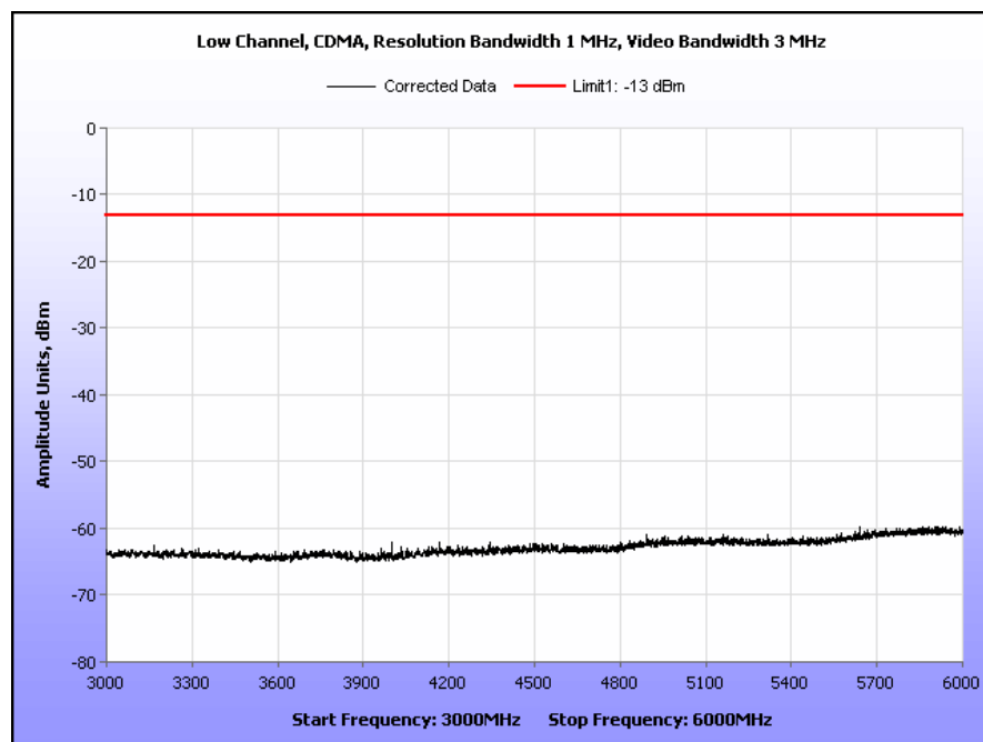
Plot 54. Radiated Spurious Emissions, Low Channel, CDMA, Part 24, 3 GHz – 6 GHz
