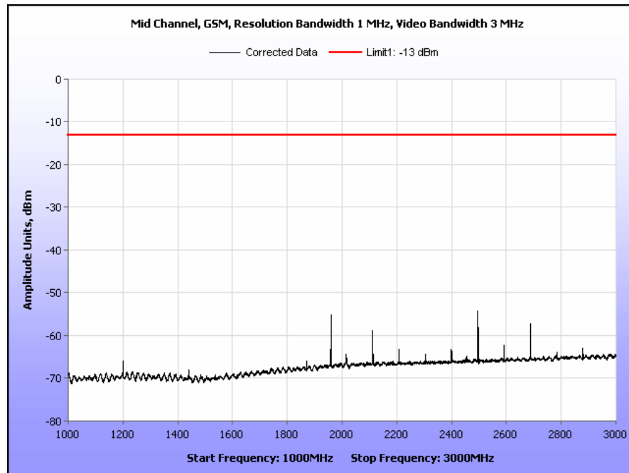
Plot 43. Radiated Spurious Emissions, Mid Channel, GSM, Part 24, 1 GHz – 3 GHz
