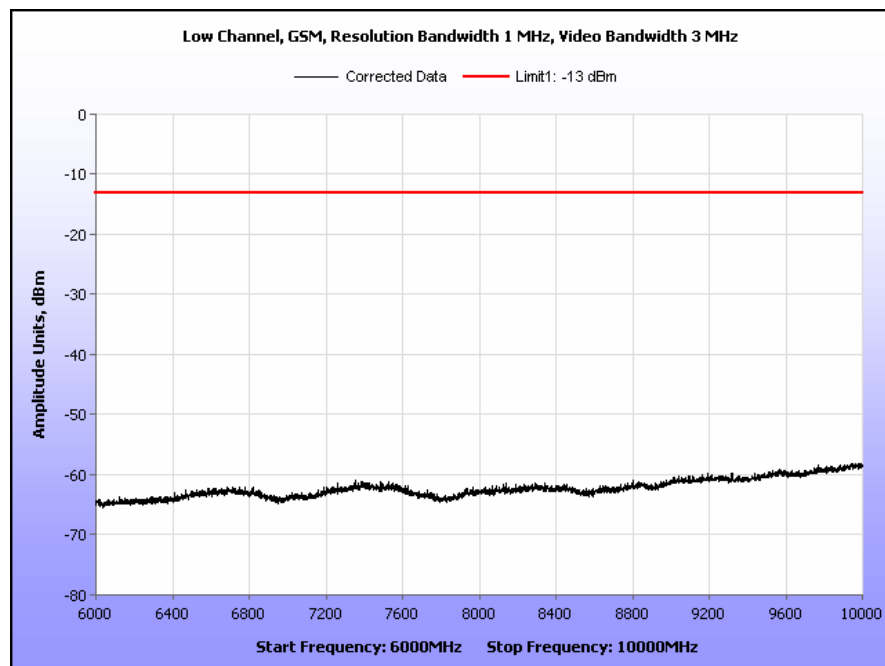
Plot 16. Radiated Spurious Emissions, Low Channel, GSM, Part 22, 6 GHz – 10 GHz
