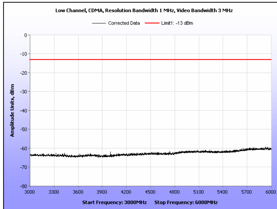
Plot 27. Radiated Spurious Emissions, Low Channel, CDMA, Part 22, 3 GHz – 6 GHz
