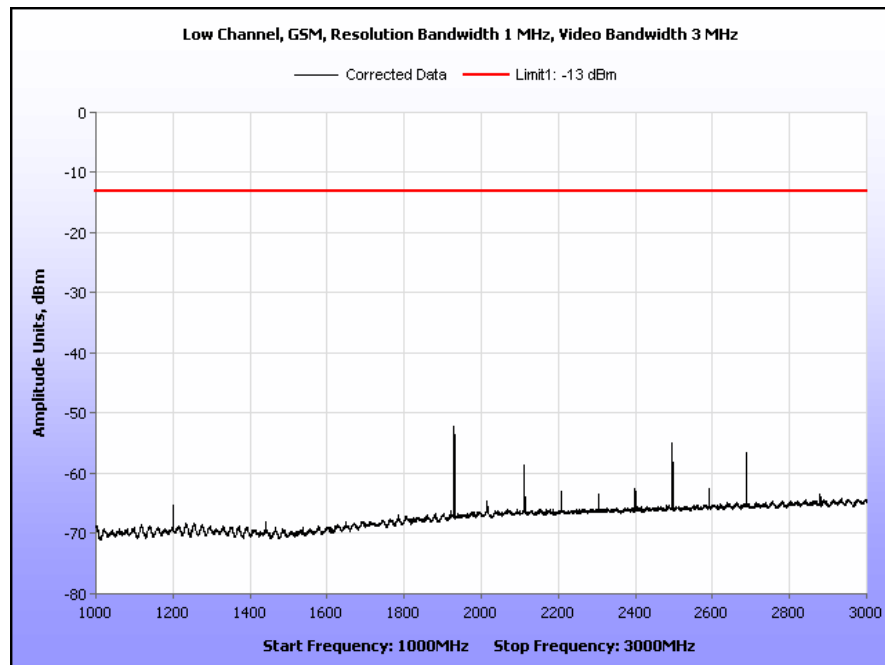
Plot 38. Radiated Spurious Emissions, Low Channel, GSM, Part 24, 1 GHz – 3 GHz
