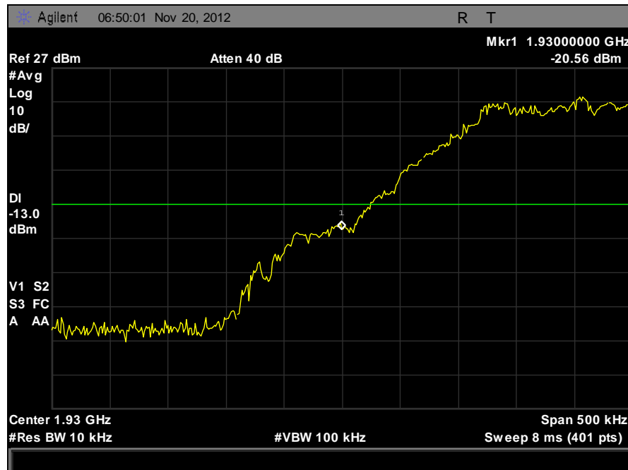
Plot 71. Band Edge, Part 24, GSM, Low Channel
