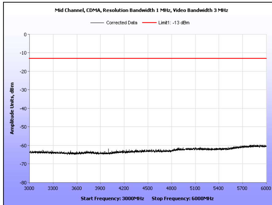
Plot 31. Radiated Spurious Emissions, Mid Channel, CDMA, Part 22, 3 GHz – 6 GHz
