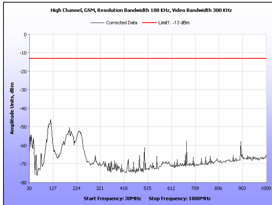
Plot 21. Radiated Spurious Emissions, High Channel, GSM, Part 22, 30 MHz – 1 GHz
