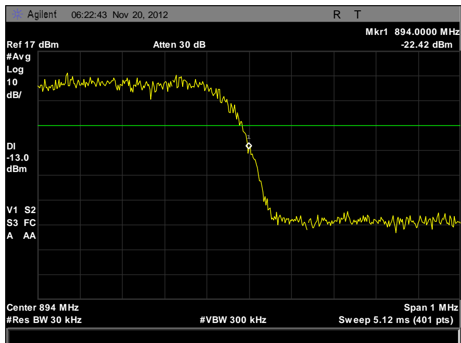
Plot 70. Band Edge, Part 22, CDMA, High Channel
