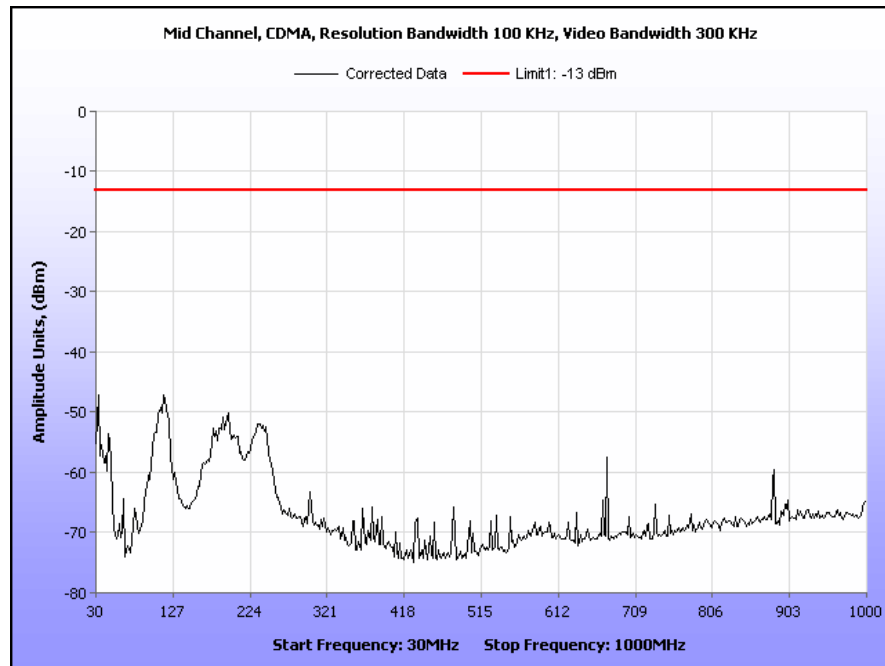
Plot 29. Radiated Spurious Emissions, Mid Channel, CDMA, Part 22, 30 MHz – 1 GHz
