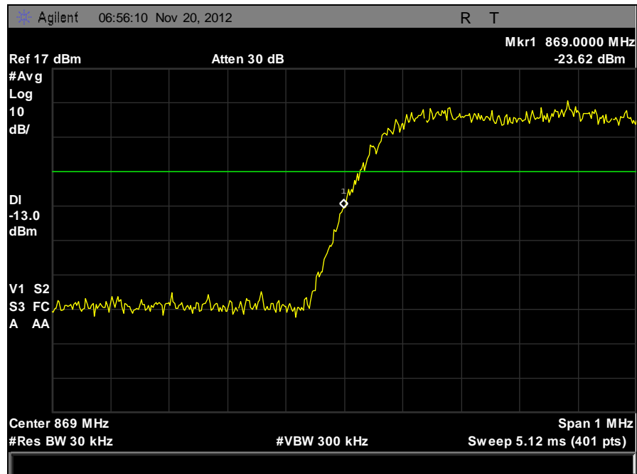
Plot 69. Band Edge, Part 22, CDMA, Low Channel
