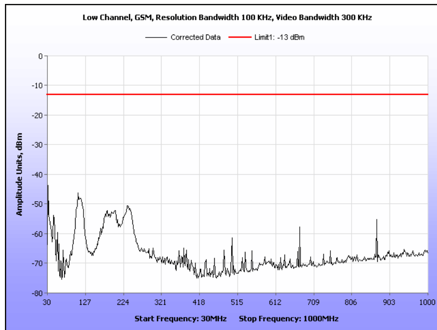
Plot 13. Radiated Spurious Emissions, Low Channel, GSM, Part 22, 30 MHz – 1 GHz
