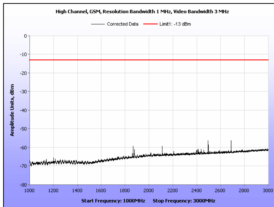
Plot 22. Radiated Spurious Emissions, High Channel, GSM, Part 22, 1 GHz – 3 GHz
