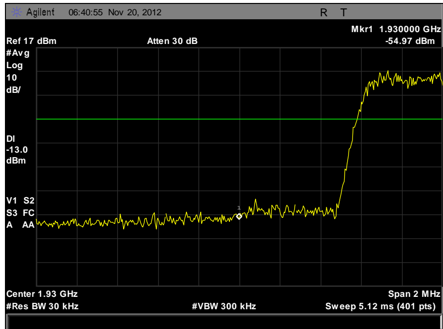
Plot 73. Band Edge, Part 24, CDMA, Low Channel
