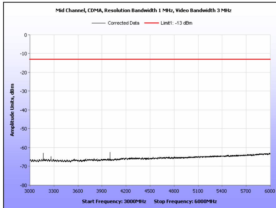
Plot 59. Radiated Spurious Emissions, Mid Channel, CDMA, Part 24, 3 GHz – 6 GHz
