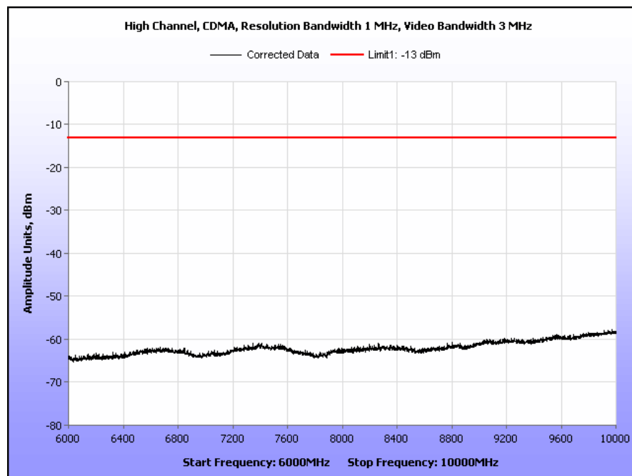
Plot 36. Radiated Spurious Emissions, High Channel, CDMA, Part 22, 6 GHz – 10 GHz
