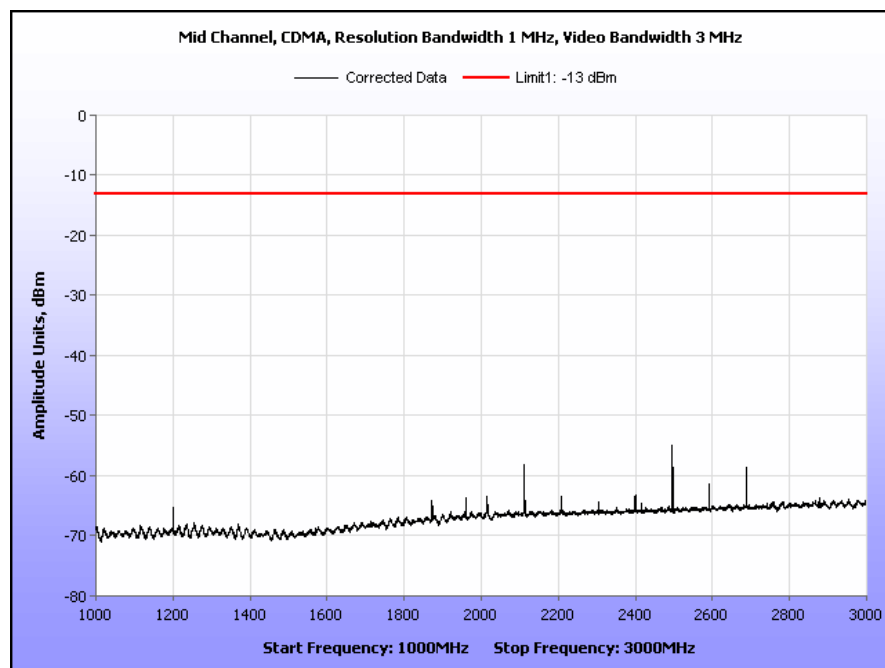
Plot 58. Radiated Spurious Emissions, Mid Channel, CDMA, Part 24, 1 GHz – 3 GHz
