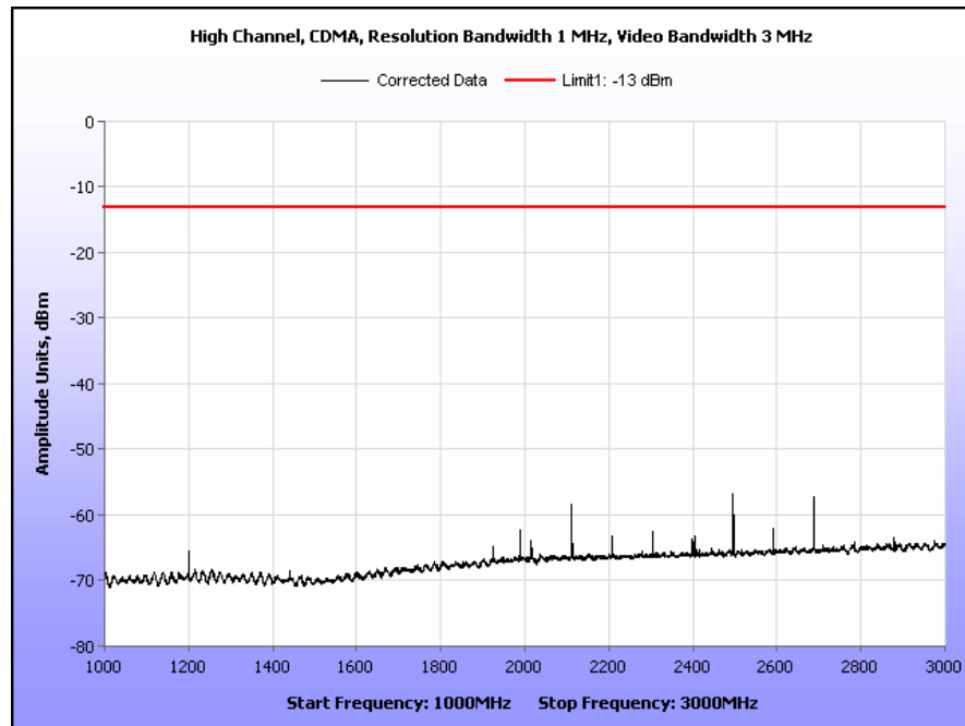
Plot 63. Radiated Spurious Emissions, High Channel, CDMA, Part 24, 1 GHz – 3 GHz
