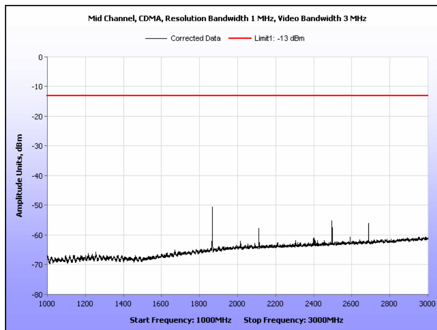
Plot 30. Radiated Spurious Emissions, Mid Channel, CDMA, Part 22, 1 GHz – 3 GHz
