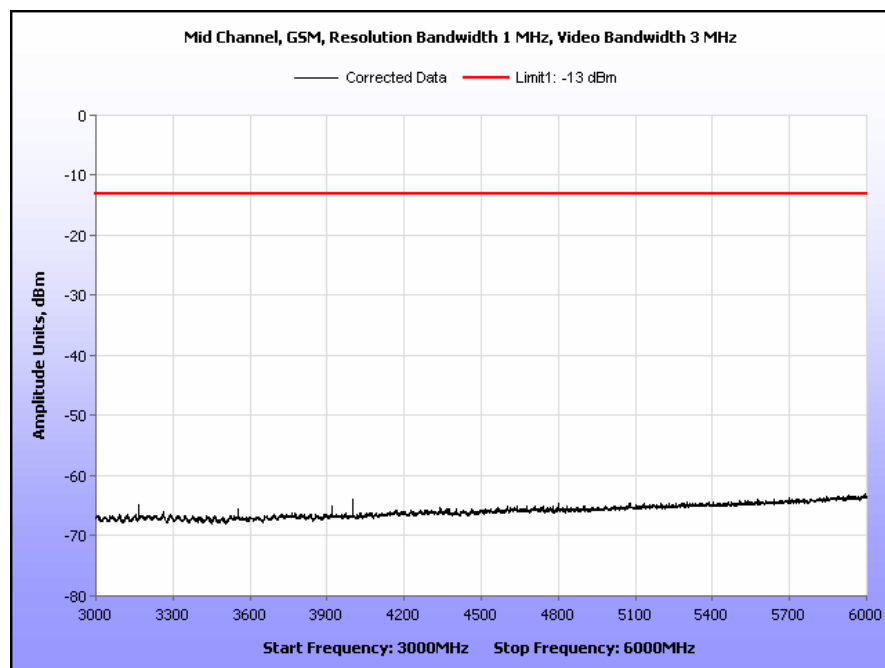
Plot 44. Radiated Spurious Emissions, Mid Channel, GSM, Part 24, 3 GHz – 6 GHz
