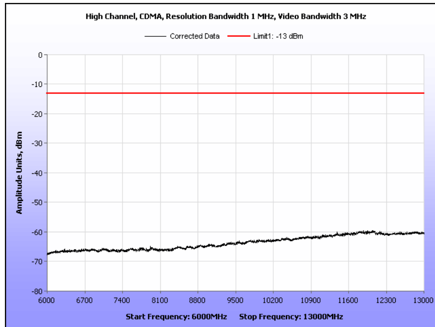
Plot 65. Radiated Spurious Emissions, High Channel, CDMA, Part 24, 6 GHz – 13 GHz
