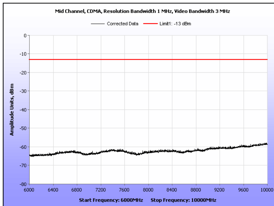
Plot 32. Radiated Spurious Emissions, Mid Channel, CDMA, Part 22, 6 GHz – 10 GHz
