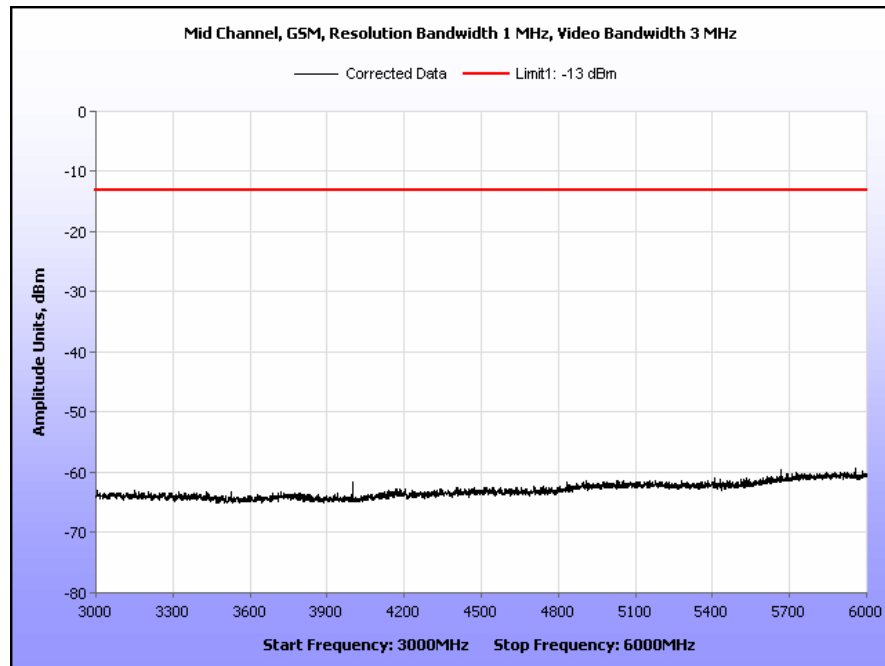
Plot 19. Radiated Spurious Emissions, Mid Channel, GSM, Part 22, 3 GHz – 6 GHz
