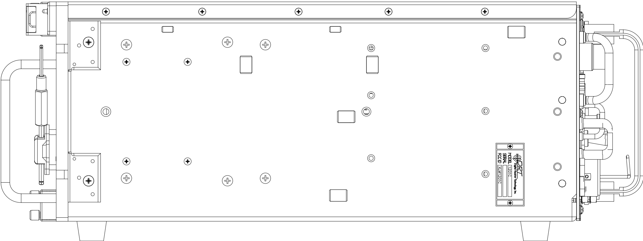
FCC Label Location Drawing For 1201C Digital Receiver Technology, Inc. 12409 Milestone Center Drive Germantown, MD 20876
