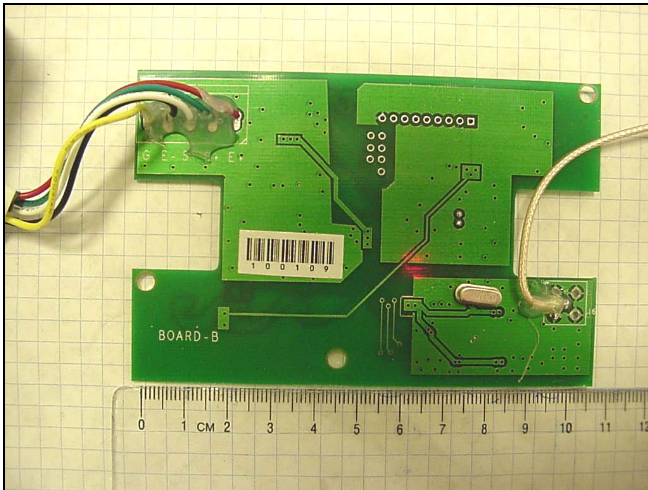
Photograph 11: Top of PCB
