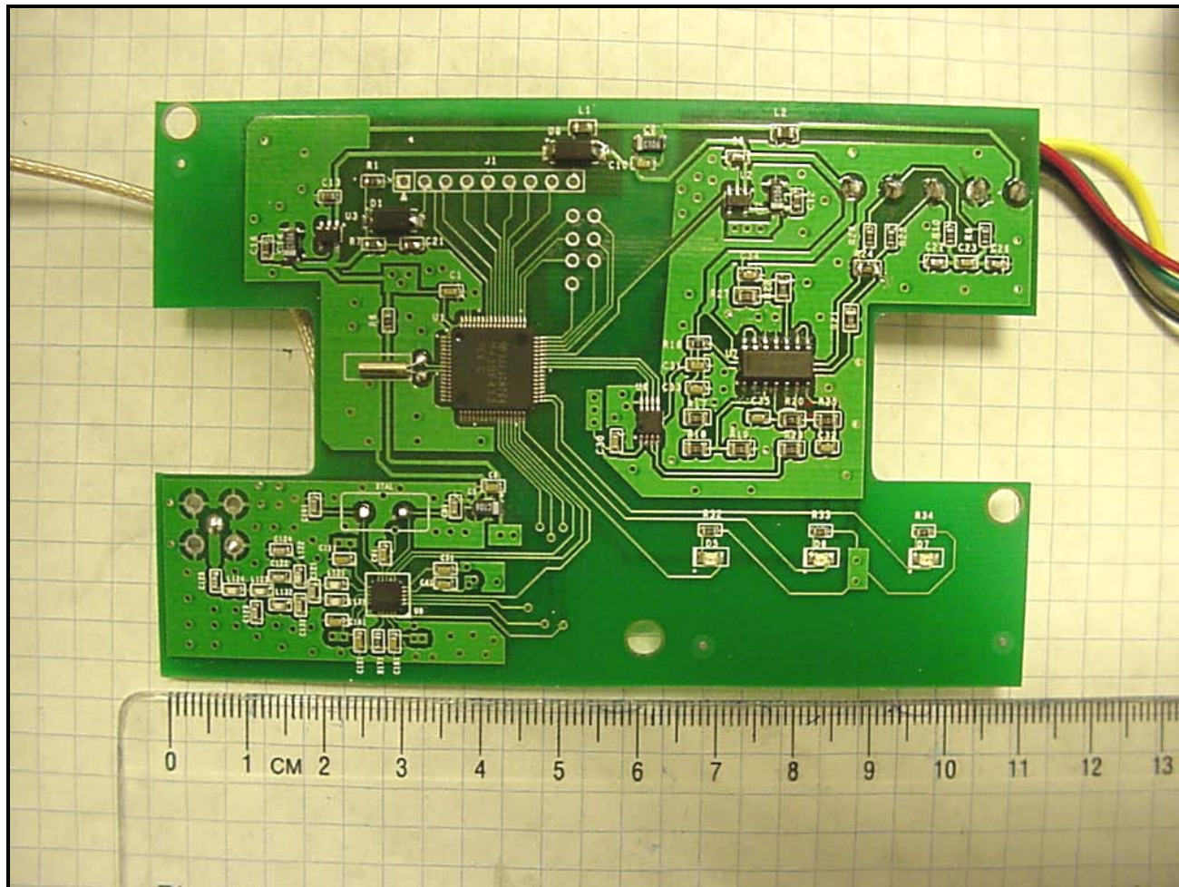
Photograph 12: Bottom of PCB
