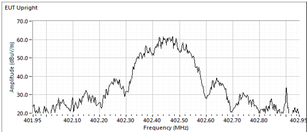
In-band with RB=3 kHz, VB=10 kHz
