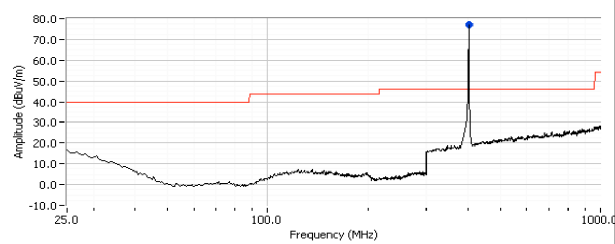
25 - 1000 MHz, Low Channel @ 402.45 MHz, EUT Upright Orientation
