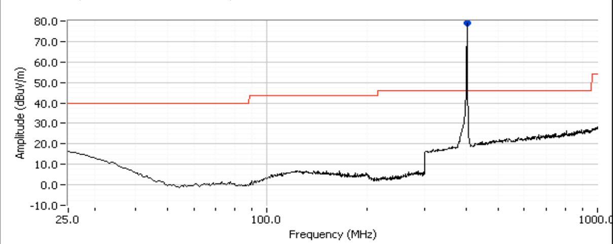
25 - 1000 MHz, Low Channel @ 402.45 MHz, EUT flat Orientation
