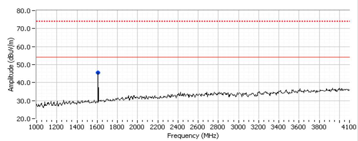
1000 - 4100 MHz, Low Channel @ 402.45 MHz, EUT Side Orientation
