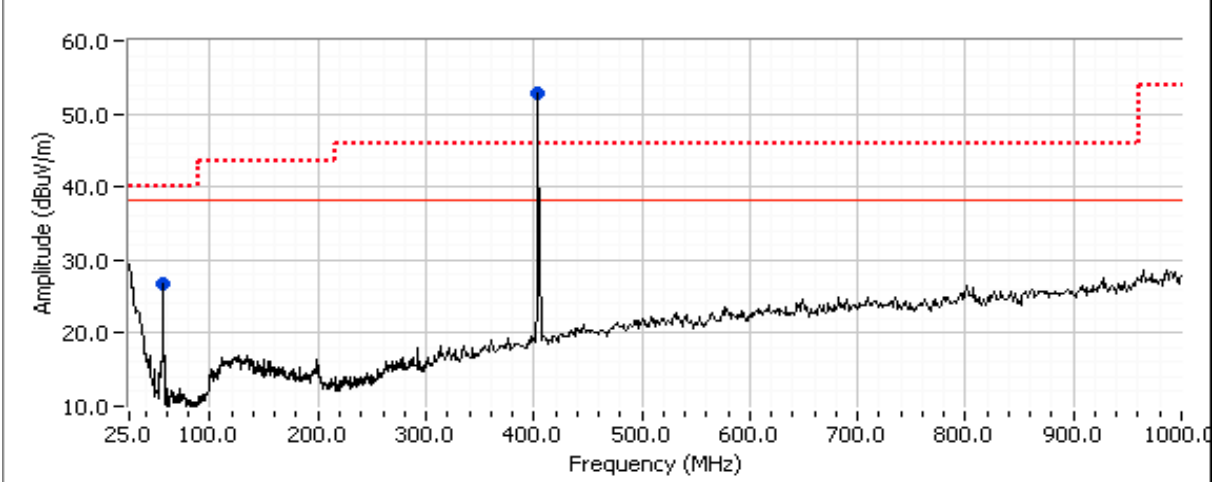
25 - 1000 MHz, High Channel @ 404.55 MHz, EUT Upright
