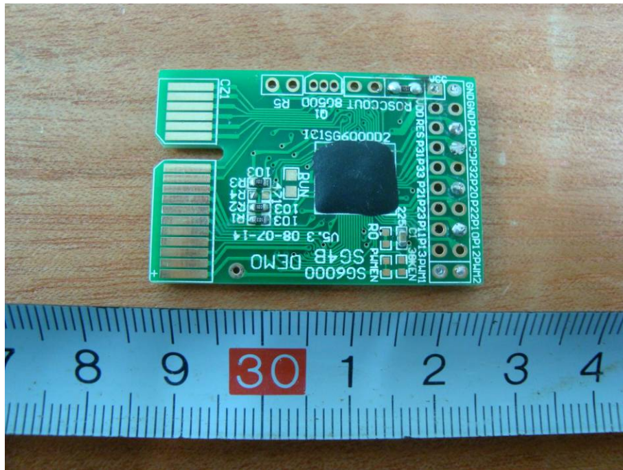
EUT – SG4B Board Components View
