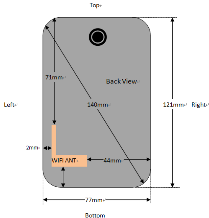
Fig.14.1 EUT Antenna Locations
