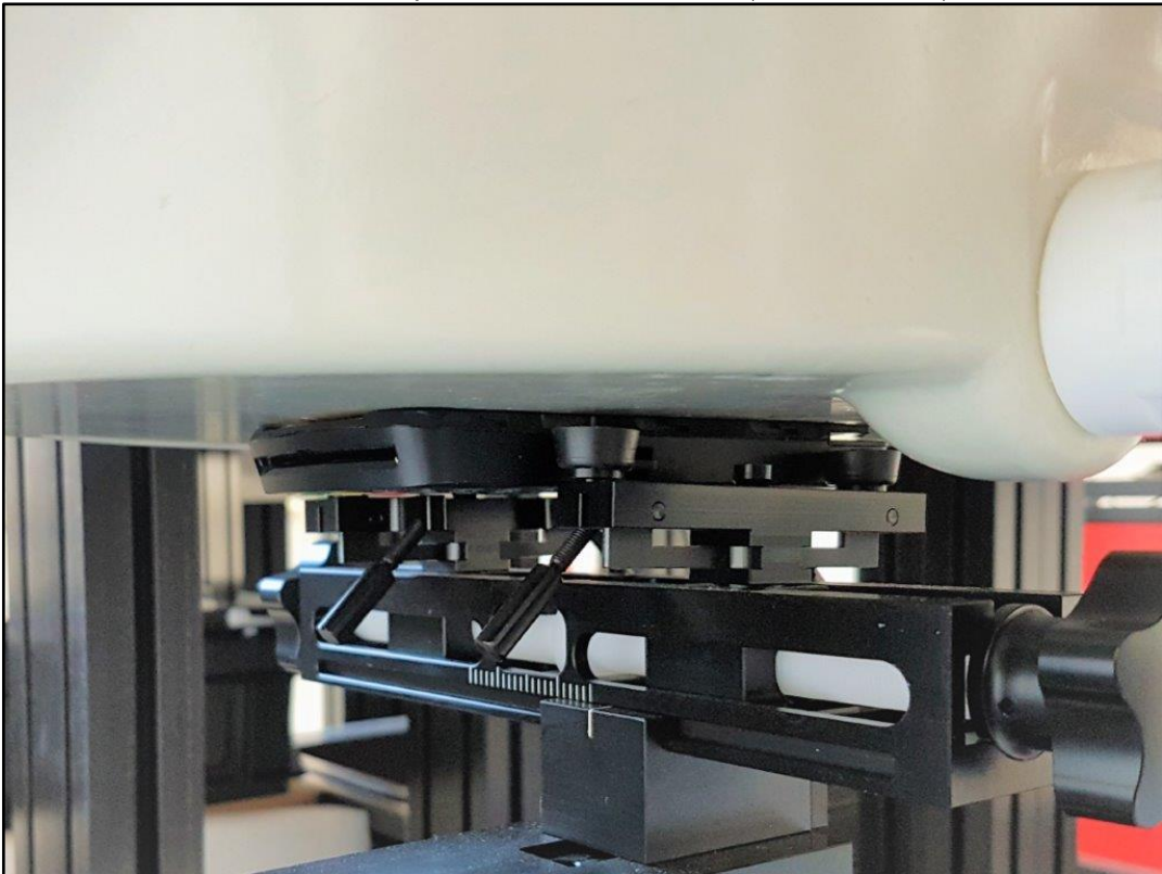
Photo 10: Test position - Back side 0mm (SAM Phantom)
