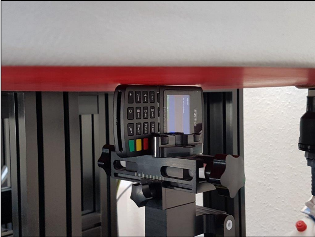
Photo 8: Test position - Top side 0mm (ELI Phantom)
