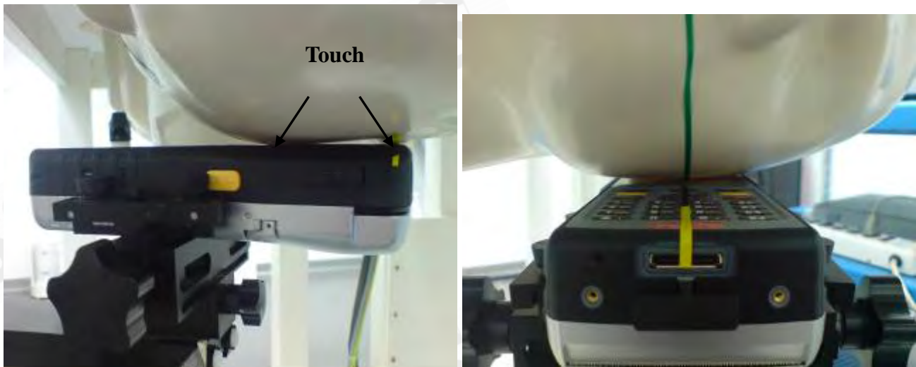
Fig.5 Left Head Section / Cheek-Touch Position
