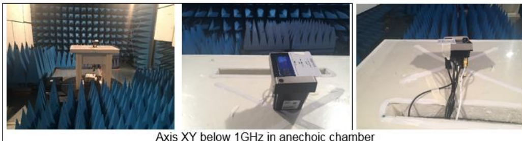
Axis XY below 1GHz in anechoic chamber
