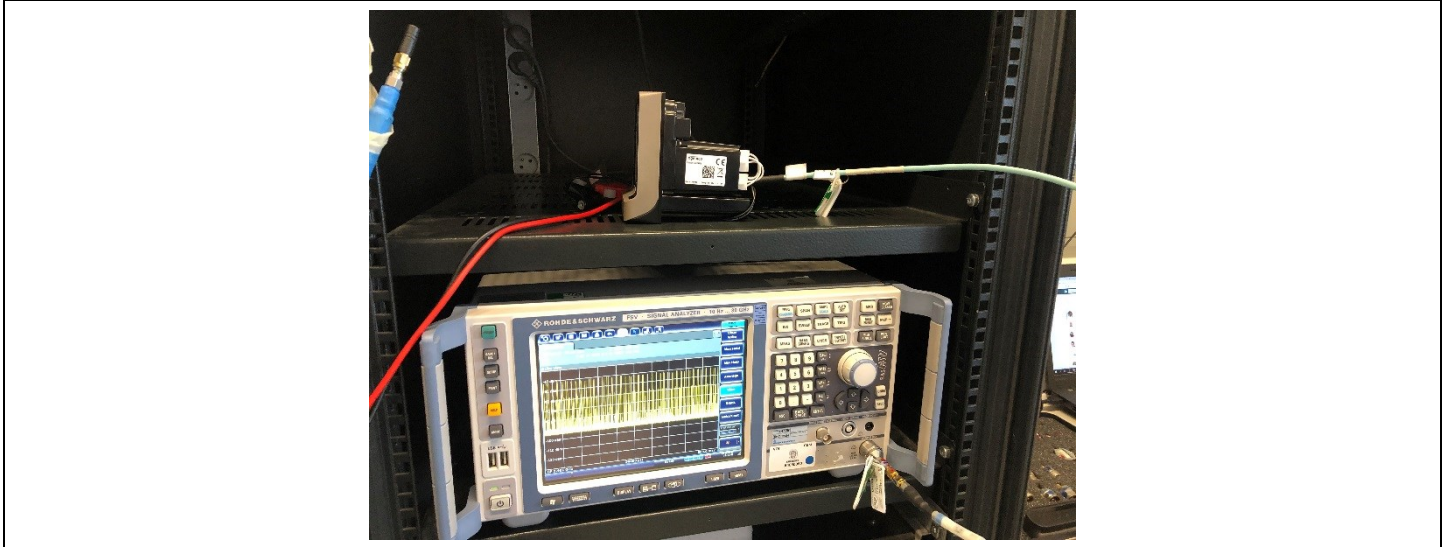
Photograph for Carrier Frequency Separation
