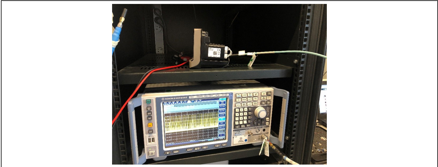
Photograph for 20dB emission bandwidth
