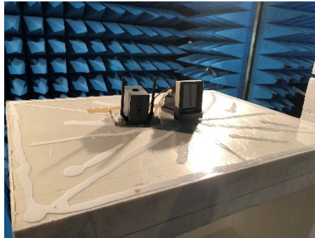
Test setup in axis XY (only one antenna position)
