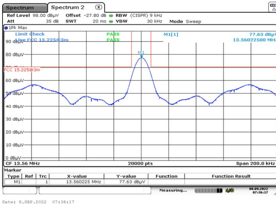
Plot 3: Spectrum mask zoomed
