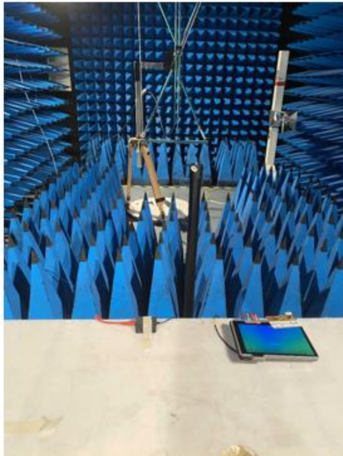
Photo in anechoic chamber – Frequency <1GHz
