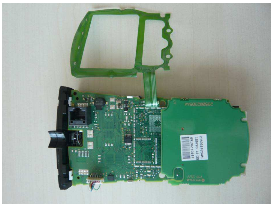
General view with antenna
