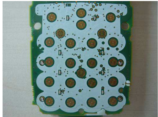
Detail views of PCB
