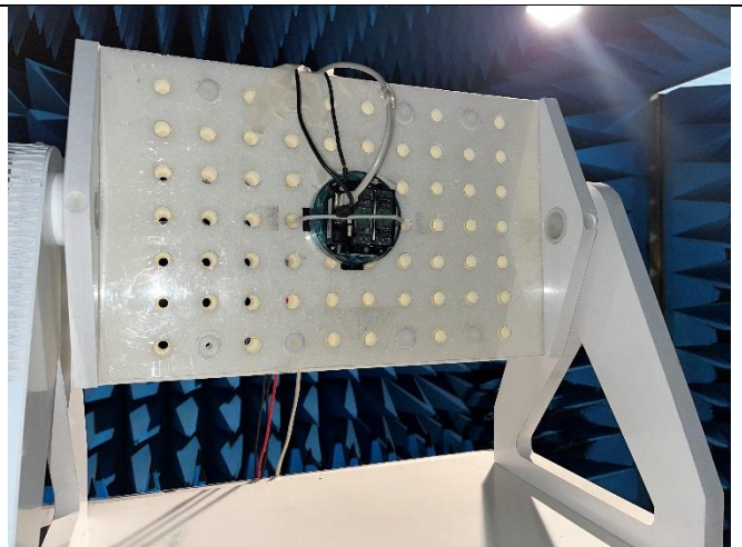
Axis Z on FAR
