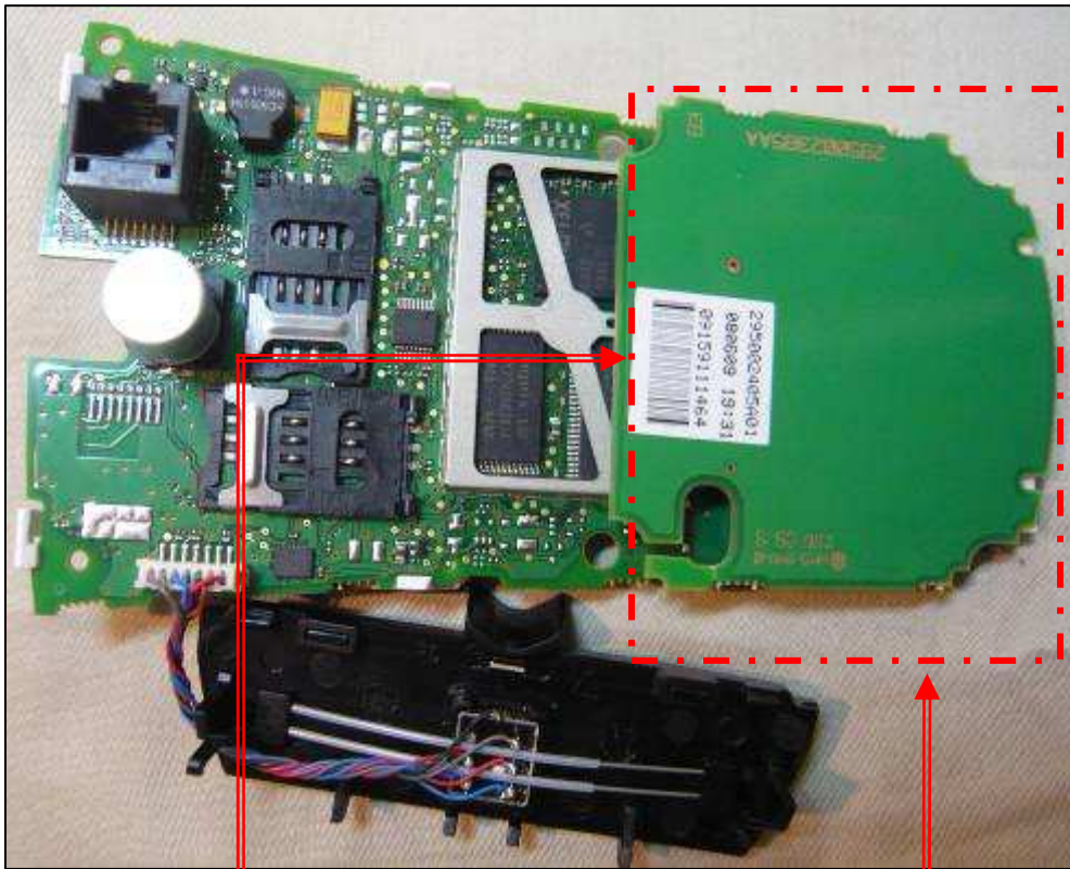
Component view, rear face
