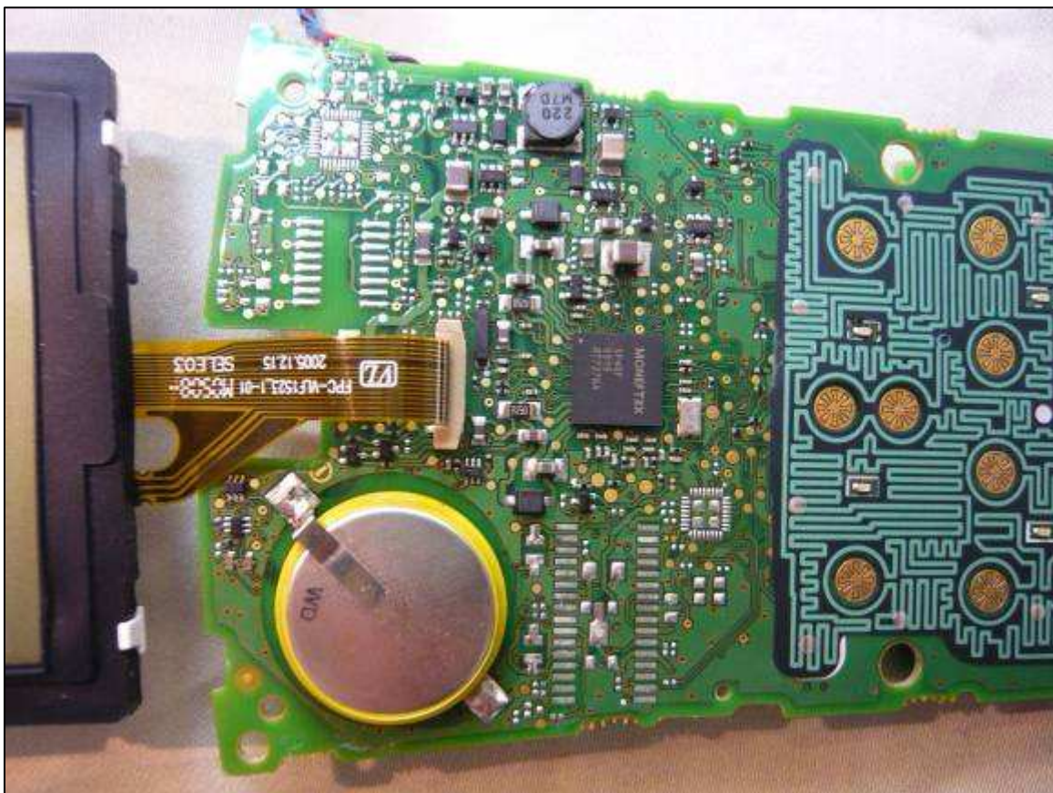
Component view, Behind LCD
