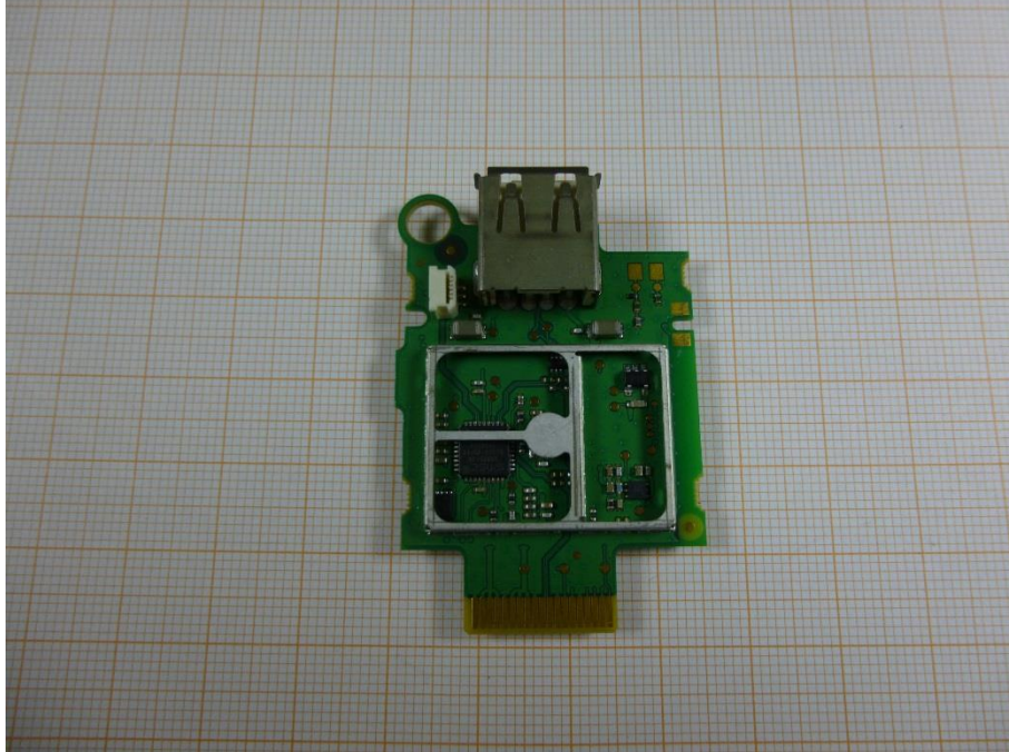
Photo 7: PCB back side view without shielding
