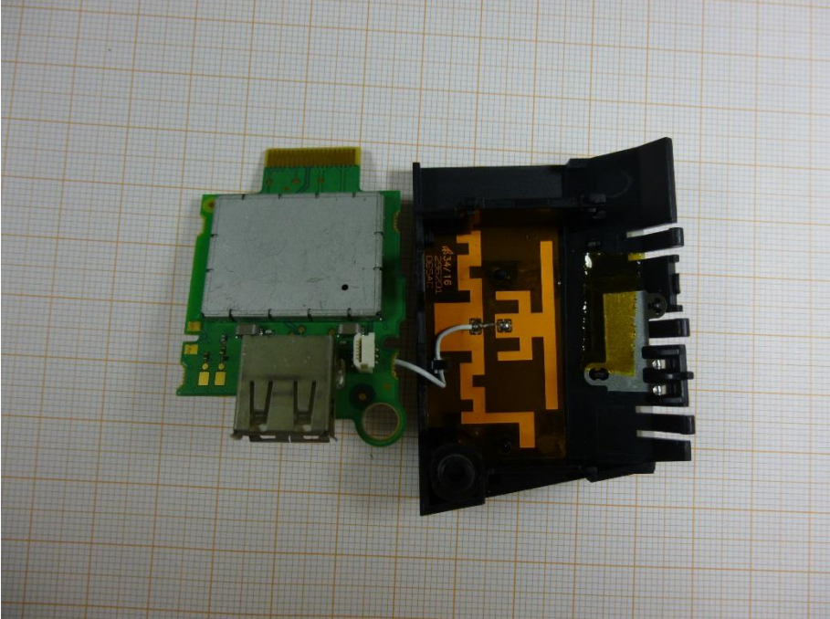
Photo 3: PCB back side view with shielding
