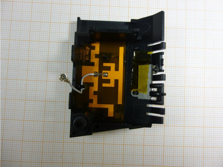
Photo 4: Antenna
