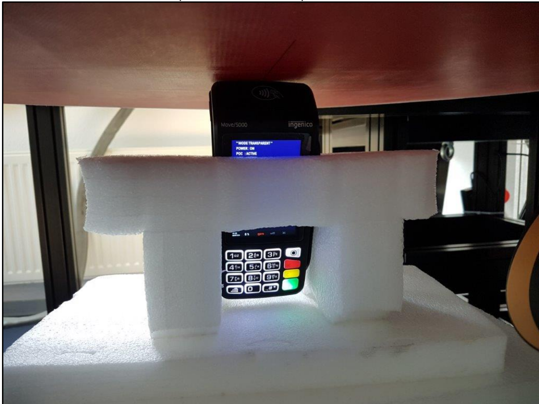
Photo 14: Test position limb worn bottom side with 0 mm distance
