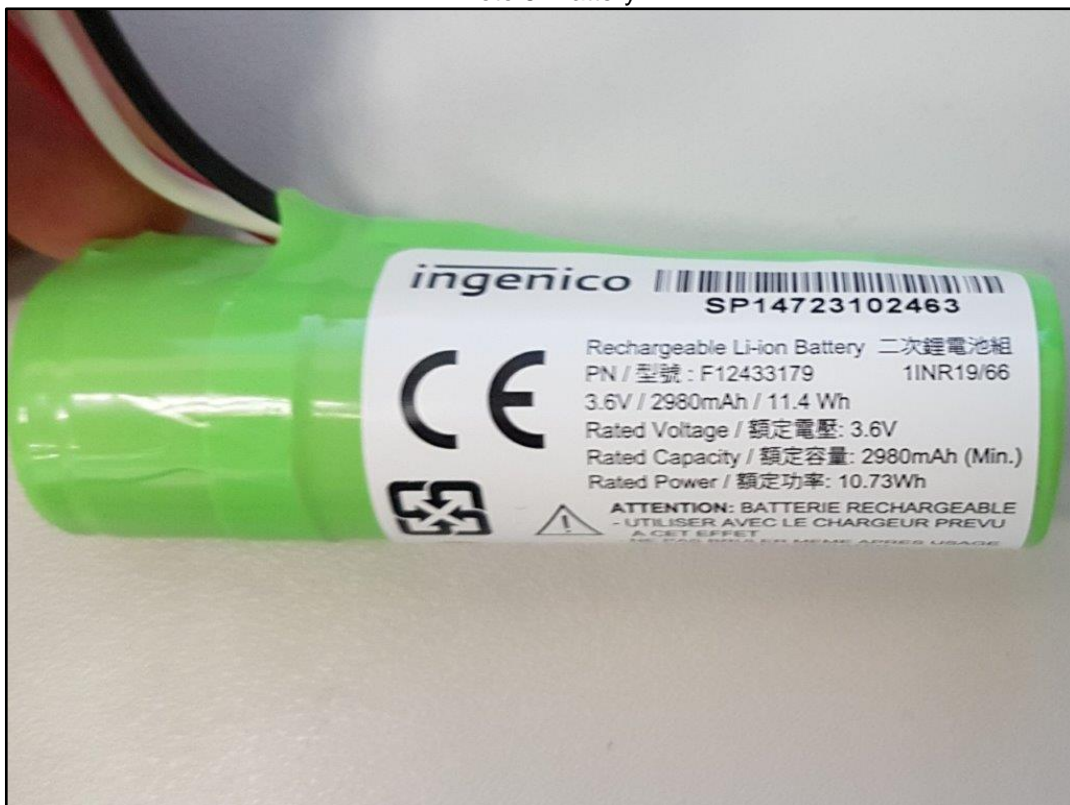
Photo 8: Battery
