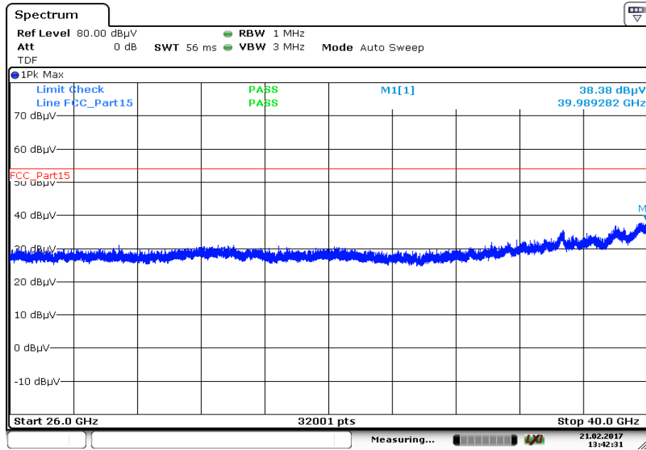
Plot 12: 26 GHz to 40 GHz, 5310 MHz, vertical & horizontal polarization
