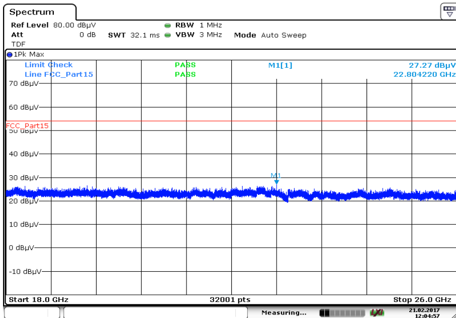
Plot 31: 18 GHz to 26 GHz, 5825 MHz, vertical & horizontal polarization
