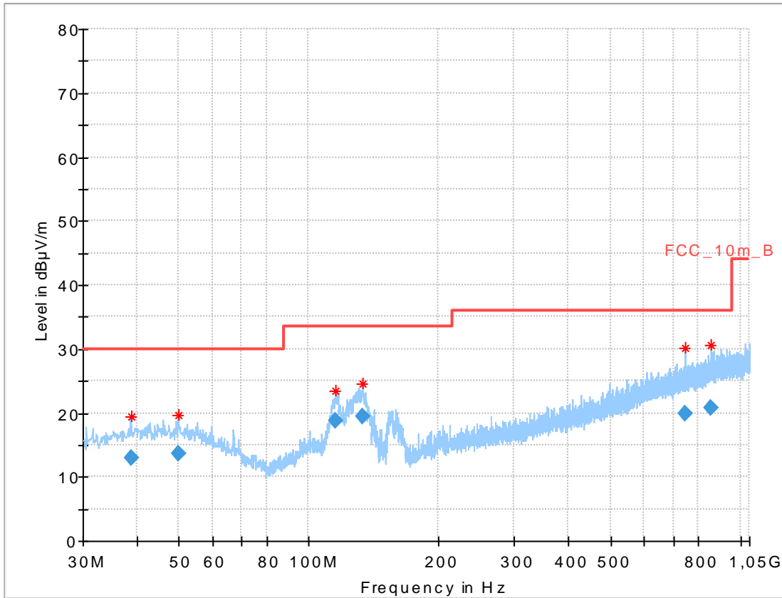
Plot 17: 30 MHz to 1 GHz, 5795 MHz, vertical & horizontal polarization
