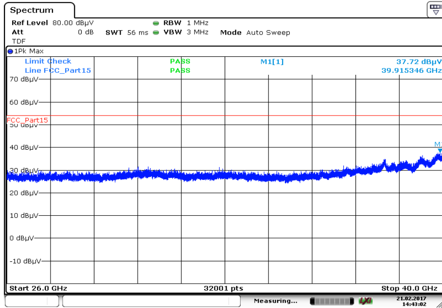
Plot 26: 26 GHz to 40 GHz, 5785 MHz, vertical & horizontal polarization
