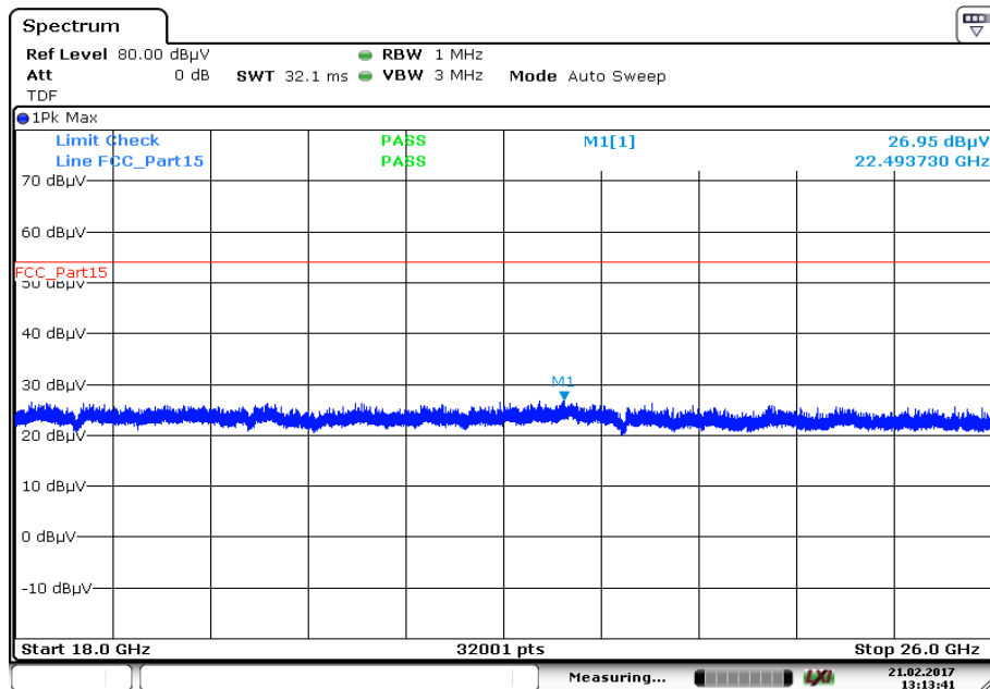
Plot 19: 18 GHz to 26 GHz, 5795 MHz, vertical & horizontal polarization
