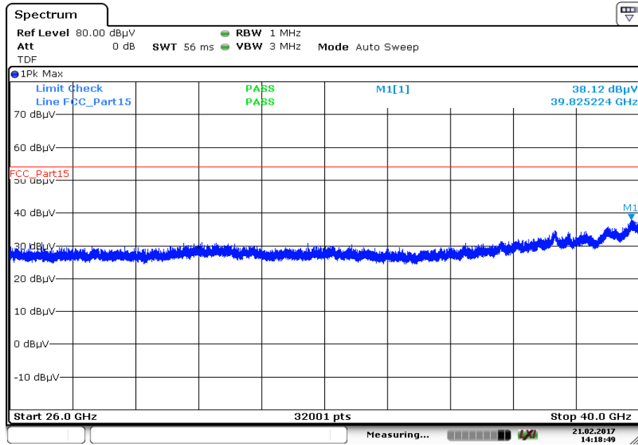
Plot 20: 26 GHz to 40 GHz, 5795 MHz, vertical & horizontal polarization
