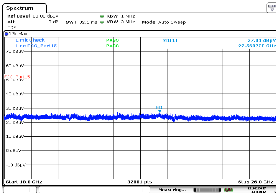
Plot 15: 18 GHz to 26 GHz, 5755 MHz, vertical & horizontal polarization
