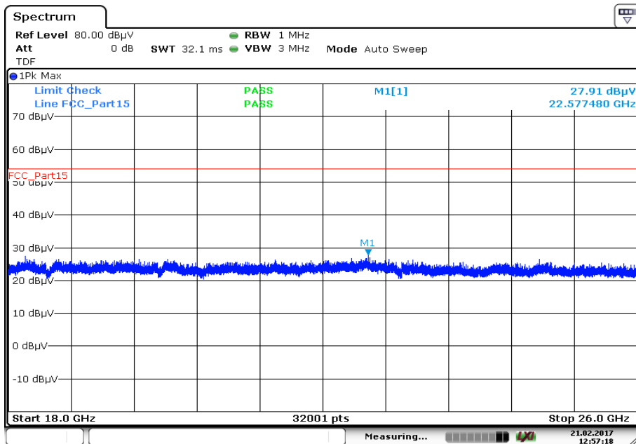
Plot 11: 18 GHz to 26 GHz, 5310 MHz, vertical & horizontal polarization
