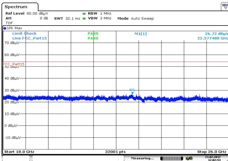
Plot 25: 18 GHz to 26 GHz, 5785 MHz, vertical & horizontal polarization
