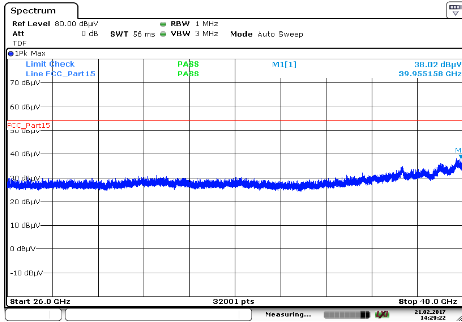
Plot 8: 26 GHz to 40 GHz, 5250 MHz, vertical & horizontal polarization
