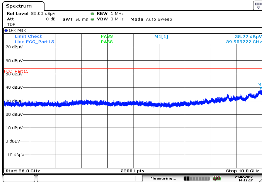
Plot 16: 26 GHz to 40 GHz, 5755 MHz, vertical & horizontal polarization
