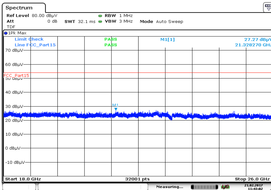
Plot 7: 18 GHz to 26 GHz, 5250 MHz, vertical & horizontal polarization
