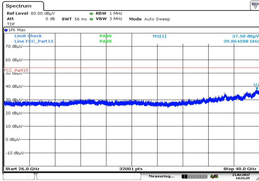
Plot 14: 26 GHz to 40 GHz, 5320 MHz, vertical & horizontal polarization
