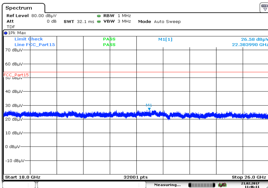
Plot 13: 18 GHz to 26 GHz, 5320 MHz, vertical & horizontal polarization
