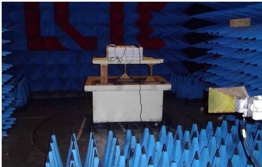
Radiated emissions measurements (above 1GHz)
