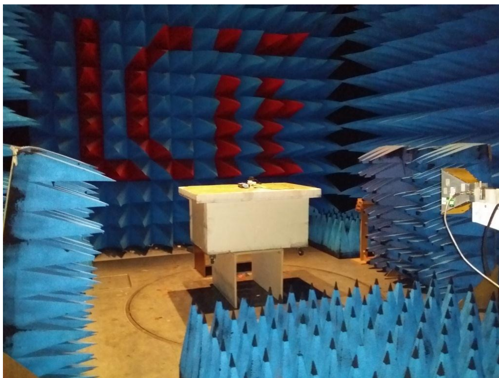
Radiated emissions measurements (above 1GHz)
