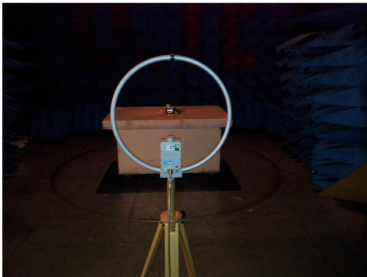
Radiated emissions measurements (below 1GHz)
