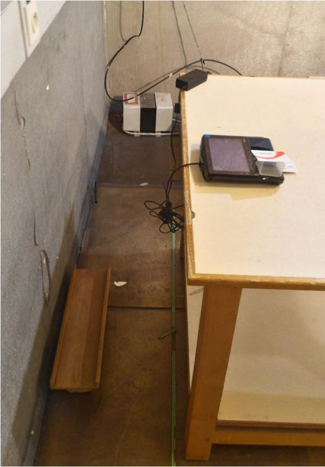
Photograph for AC Power Line Conducted Emissions (Rear view)
