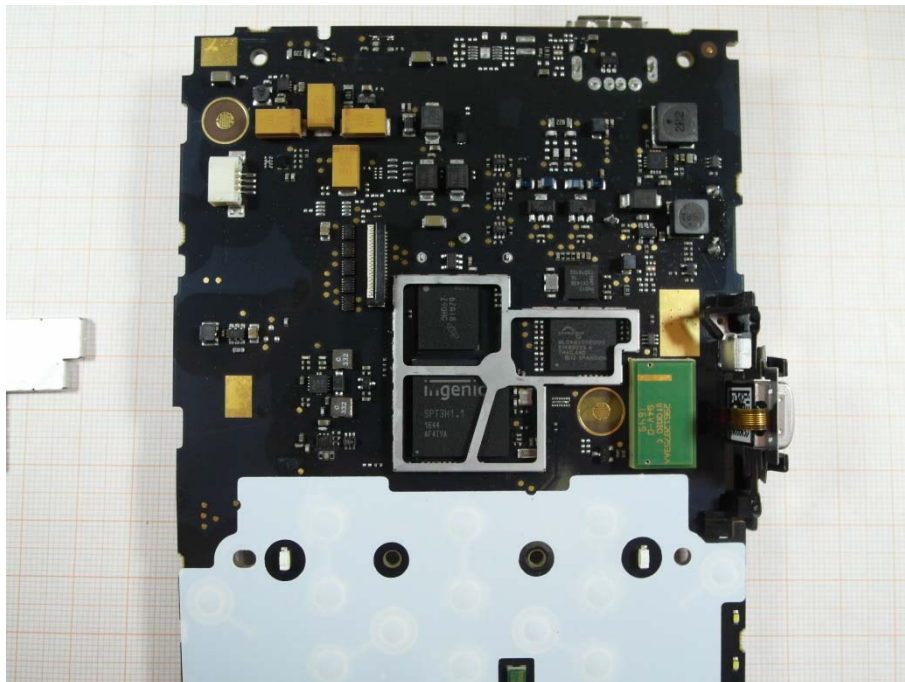
Photo 12: Shield removed
