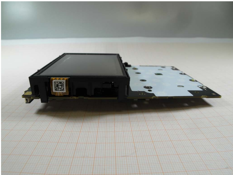
Photo 8: Left side view on PCB with display
