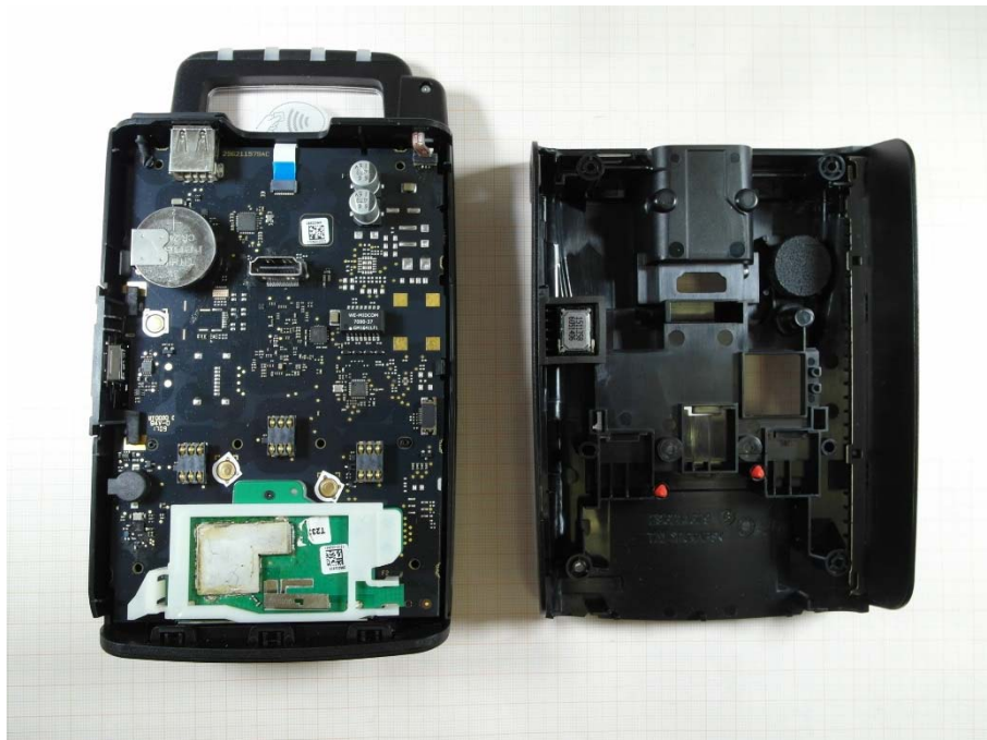
Photo 2: Bottom side back cover removed
