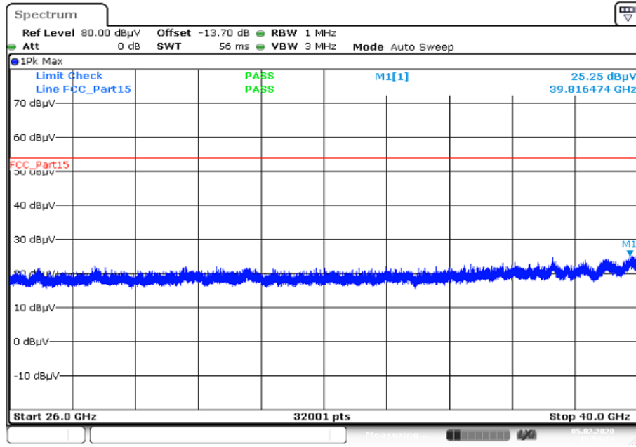
Plot 27: 26 GHz to 40 GHz; vertical & horizontal polarization; U-NII-3; middle channel
