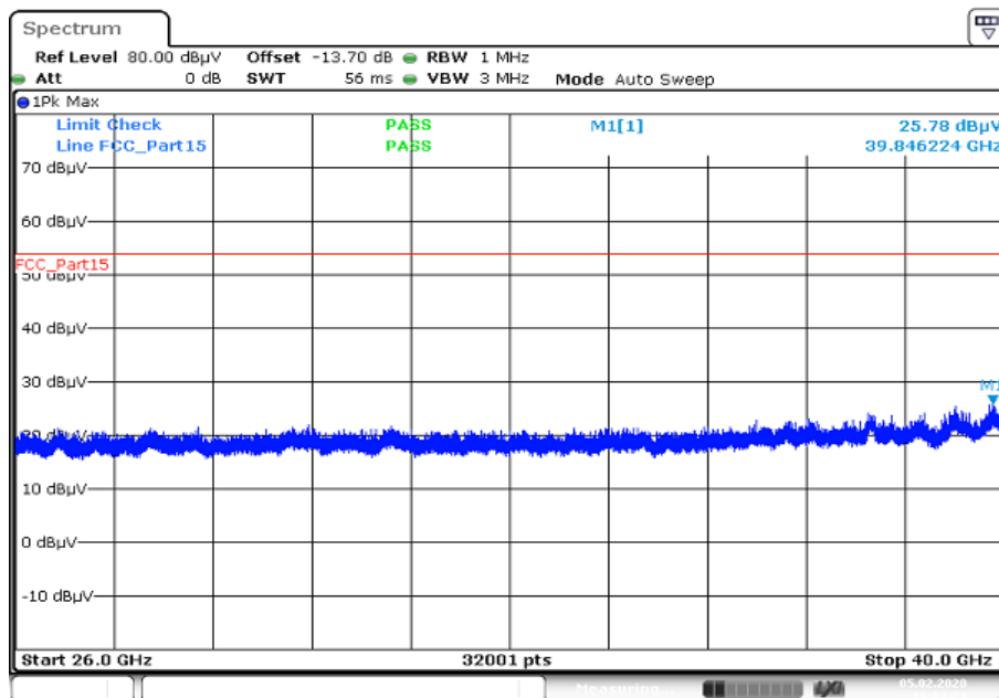
Plot 33: 26 GHz to 40 GHz, 5825 MHz, vertical & horizontal polarization, cabinet radiation
