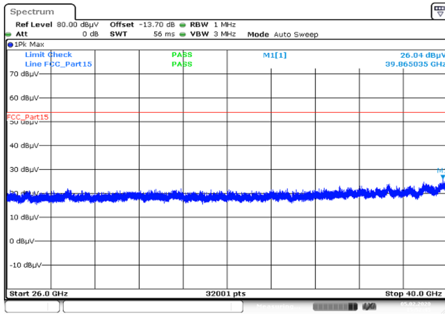
Plot 21: 26 GHz to 40 GHz; vertical & horizontal polarization; U-NII-2C; highest channel
