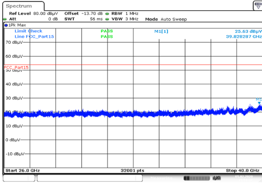
Plot 15: 26 GHz to 40 GHz; vertical & horizontal polarization; U-NII-2C; lowest channel
