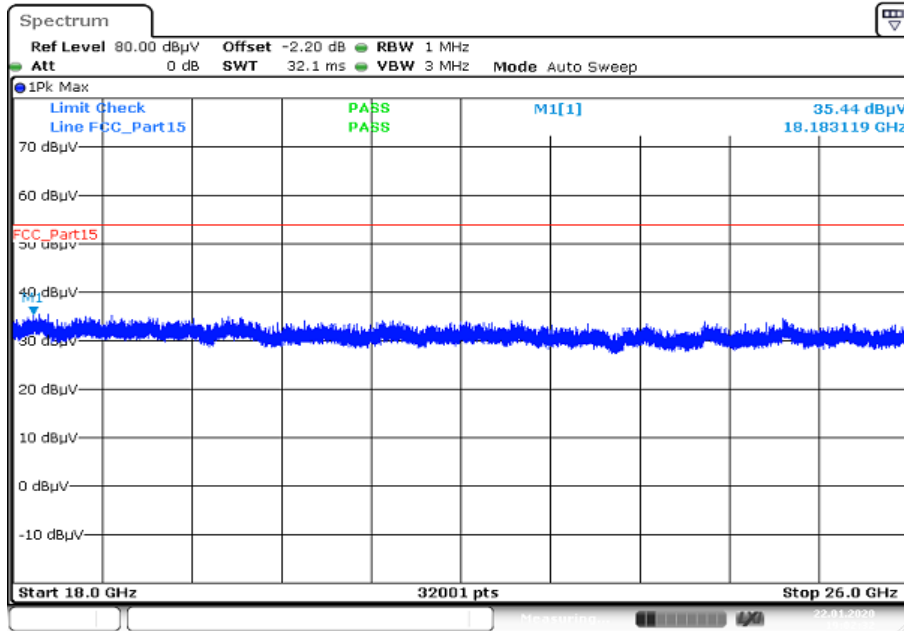
Plot 32: 18 GHz to 26 GHz, 5825 MHz, vertical & horizontal polarization, cabinet radiation
