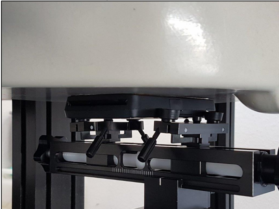
Photo 10: Test position front side with 0 mm distance
