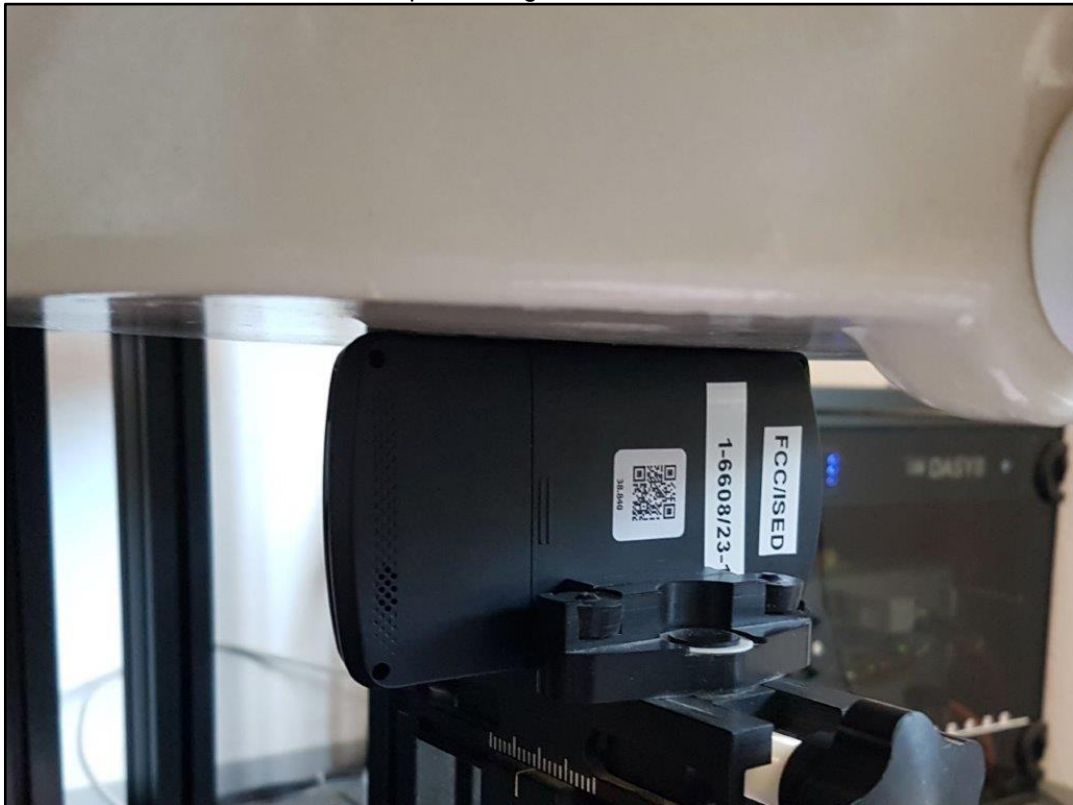
Photo 14: Test position top side with 0 mm distance
