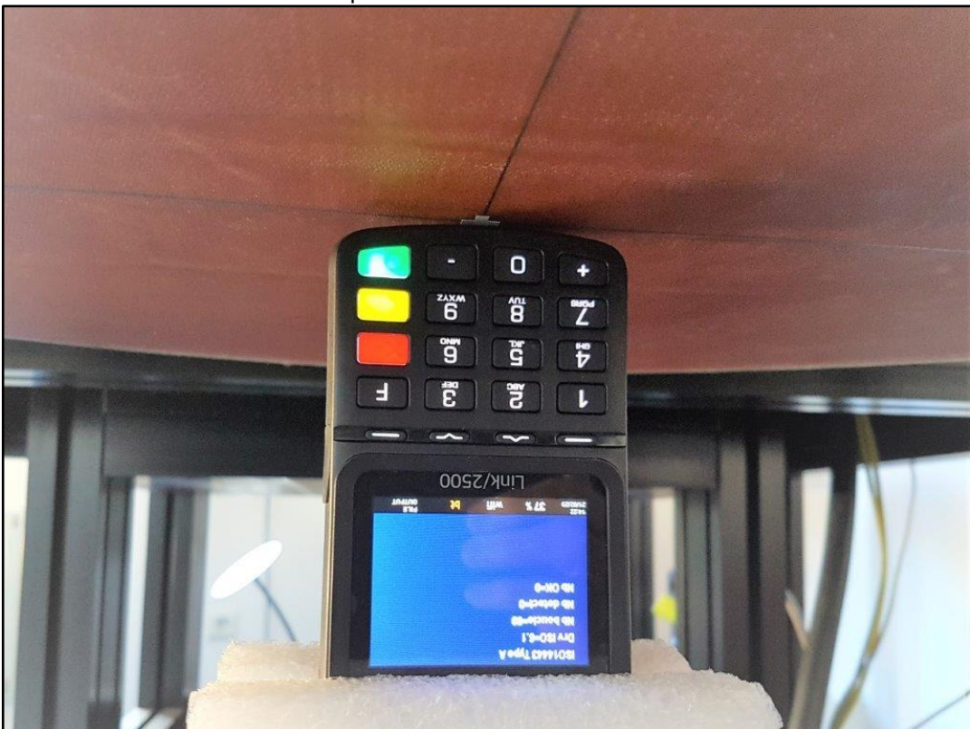
Photo 12: Test position - Bottom side with 0mm distance
