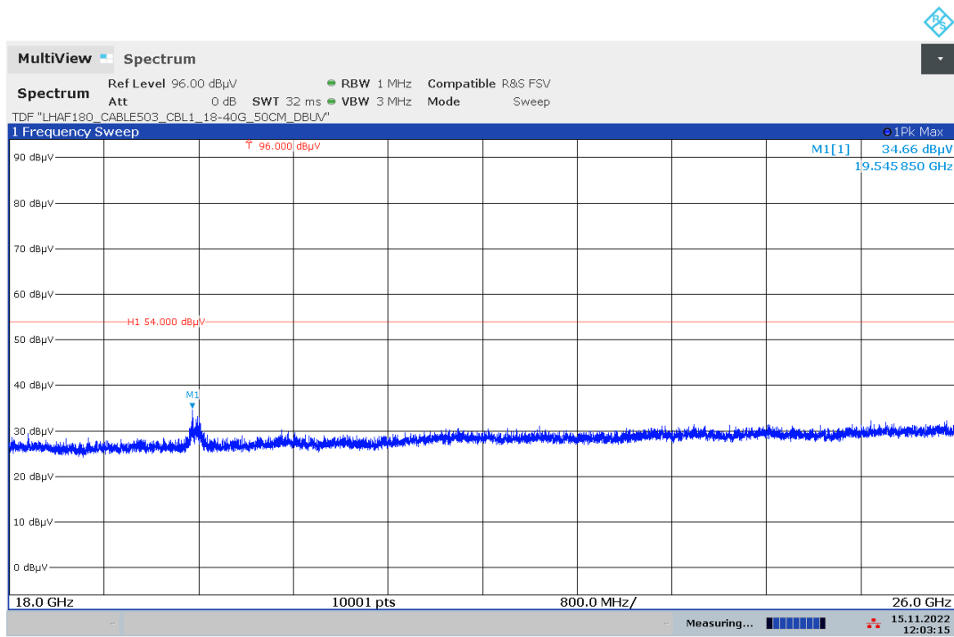
Plot 6: Three channels max hold, 18 GHz to 26 GHz, vertical & horizontal polarization
