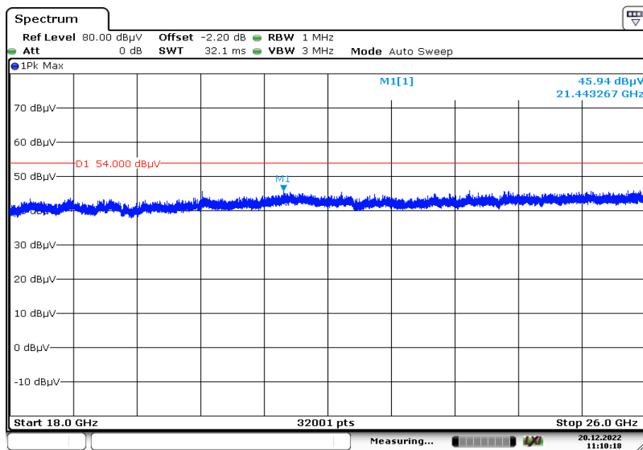
Plot 4: 18 GHz to 26 GHz, TX mode, vertical & horizontal polarization, valid for all channels and modulations
