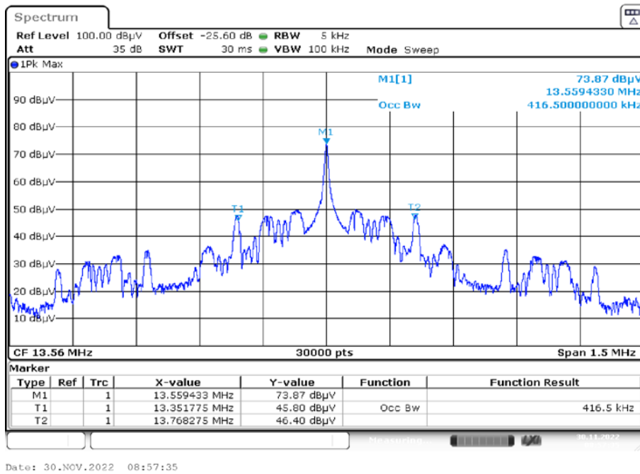
Plot 2: 99 % emission bandwidth, mode 2
