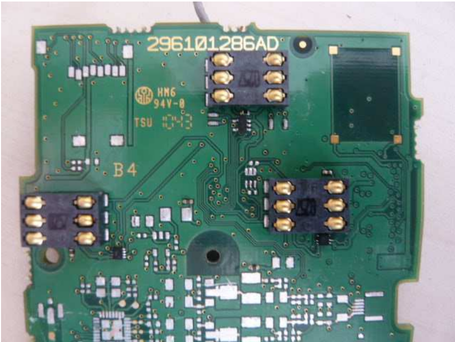
Detail views of PCB (GPRS module)
