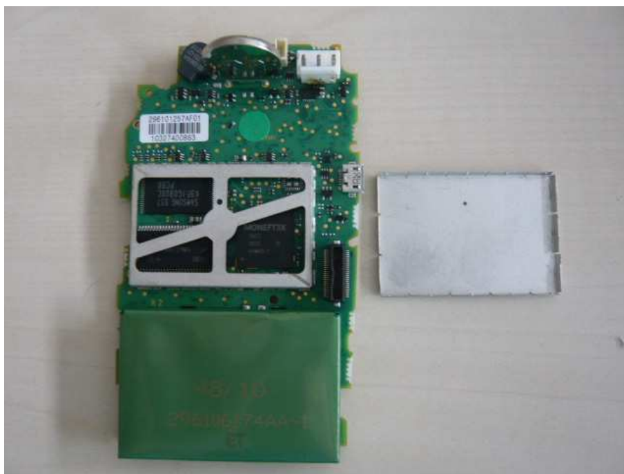
General vie of PCB without shield
