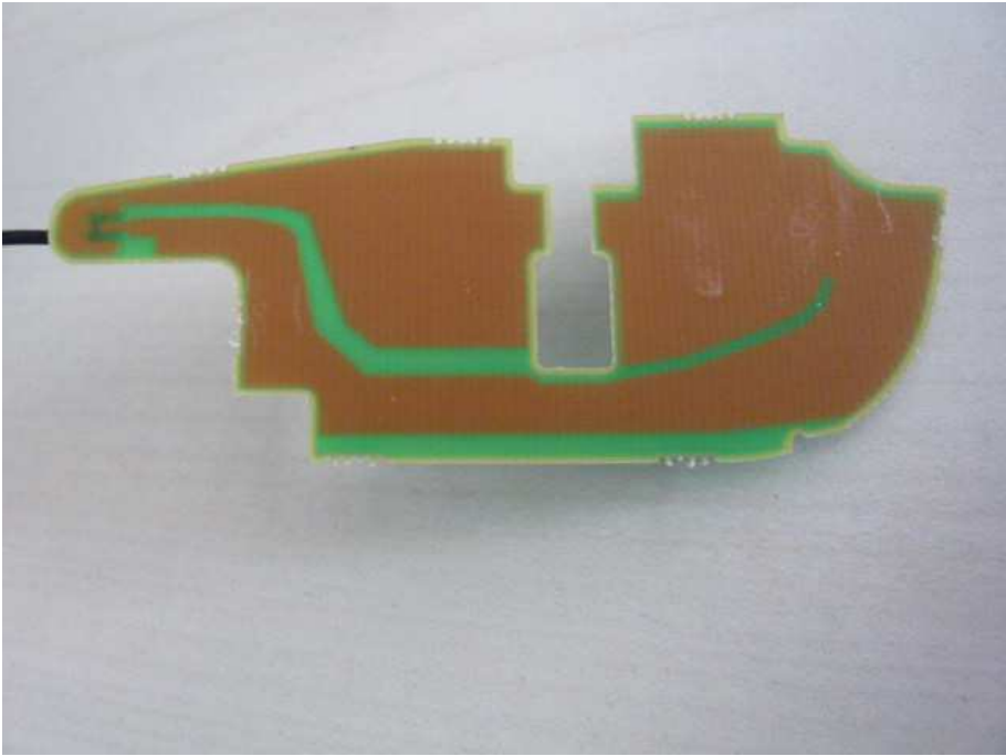
Detail views of antenna (GPRS module)
