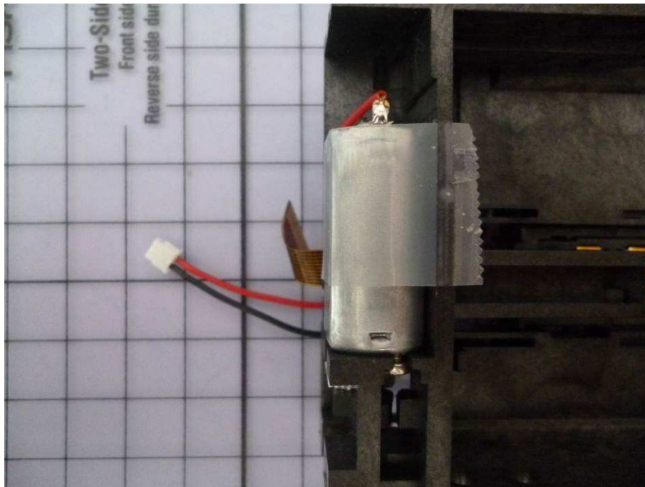
Motor for blocking card (optional, just removed for option without)
