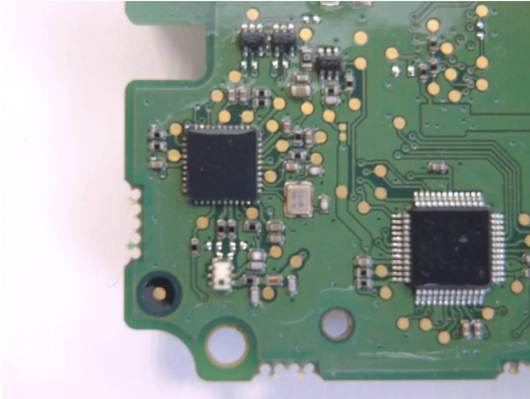
BLUETOOTH PART
