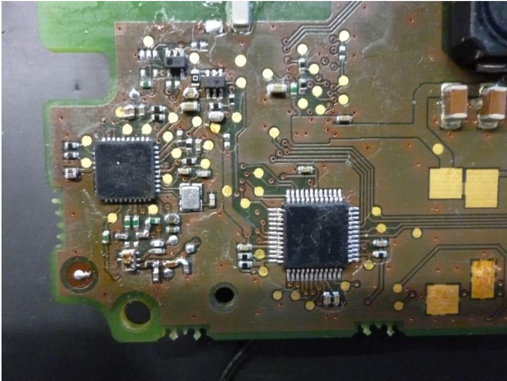
BLUETOOTH PART
