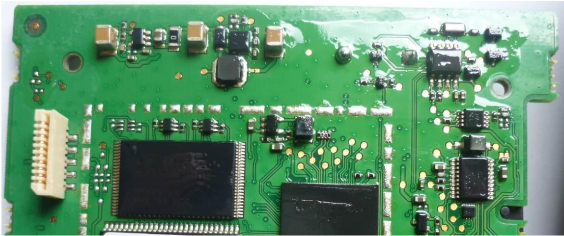
Detail views of PCB
