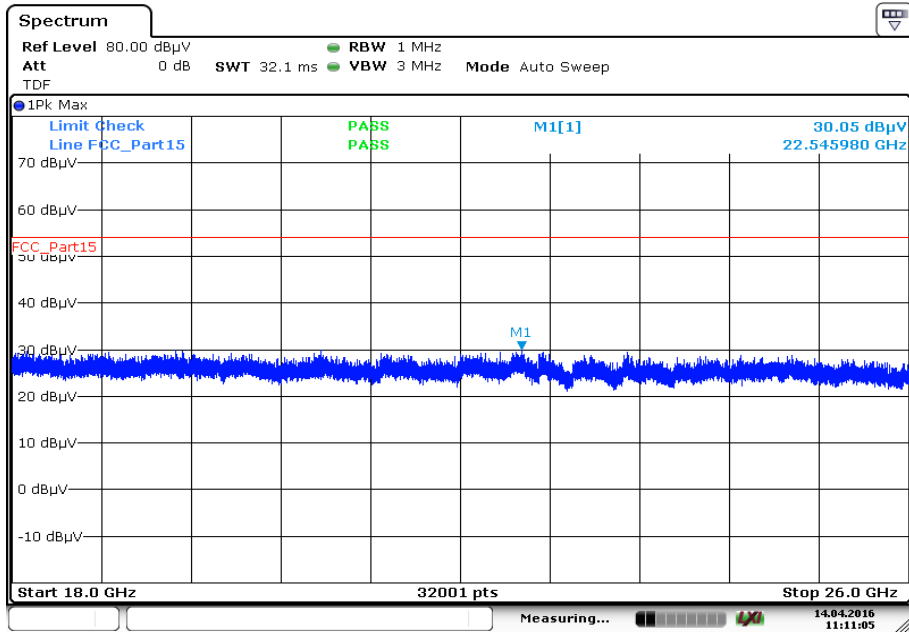
Plot 9: 18 GHz to 26 GHz, TX mode, GFSK, channel 78, vertical & horizontal polarization
