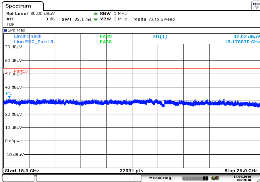
Plot 5: 18 GHz to 26 GHz, RX / idle – mode, vertical & horizontal polarization
