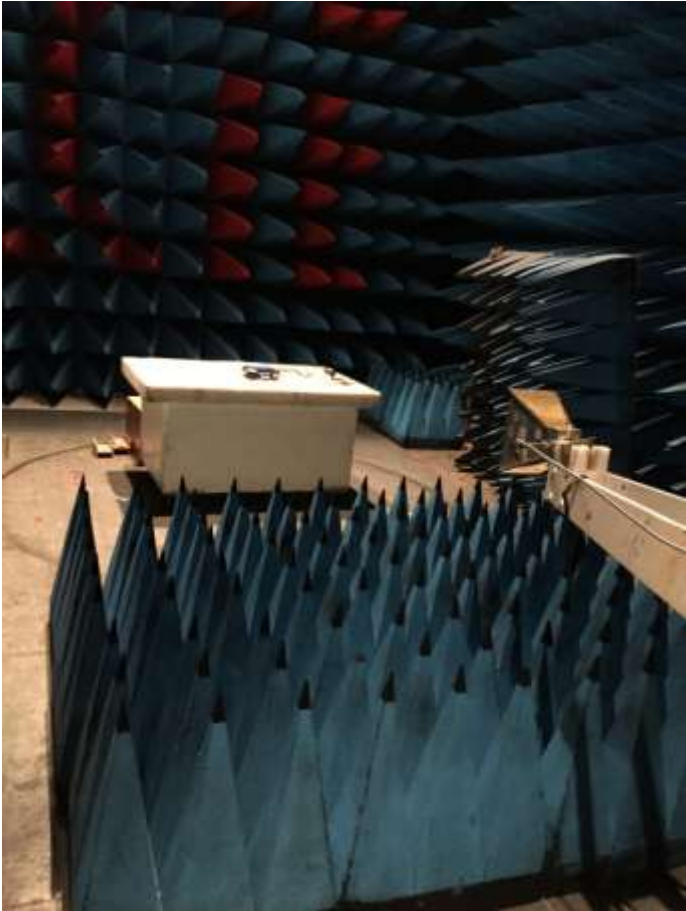
Radiated emissions measurements
