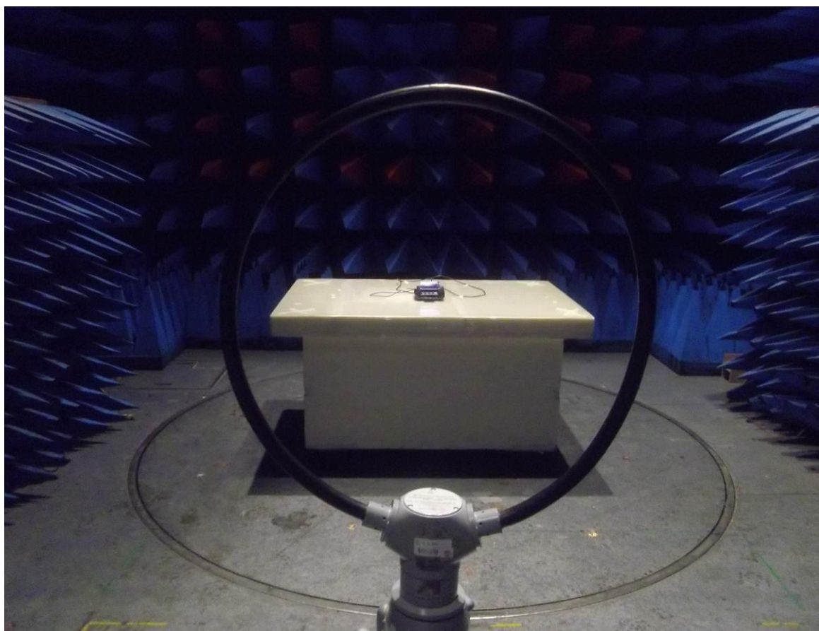
Radiated emissions measurements
