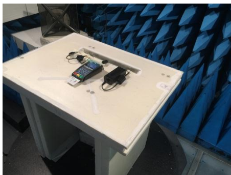
General Test setup in anechoic chamber
