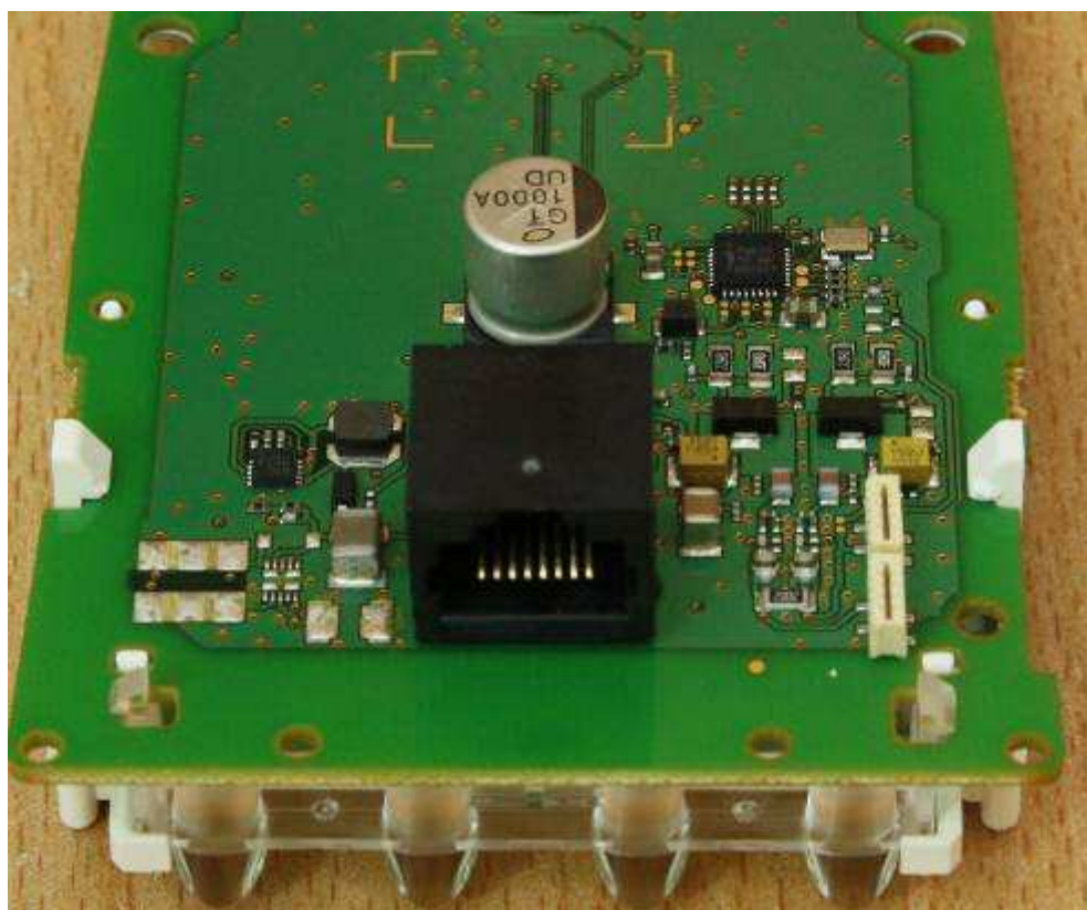
Detail views of PCB
