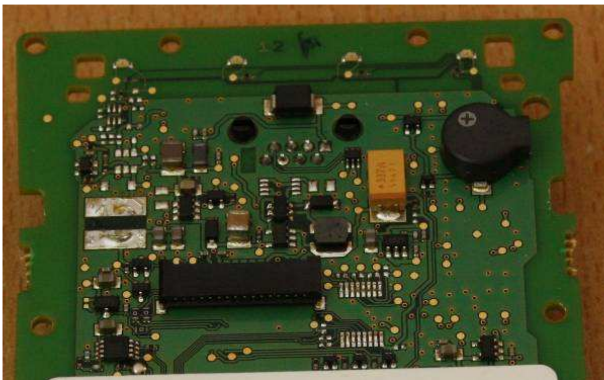
Detail views of PCB
