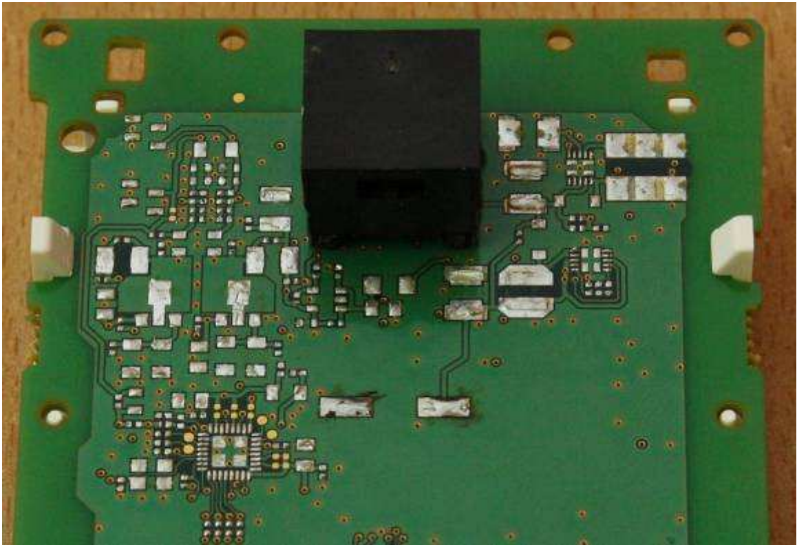
Detail views of PCB
