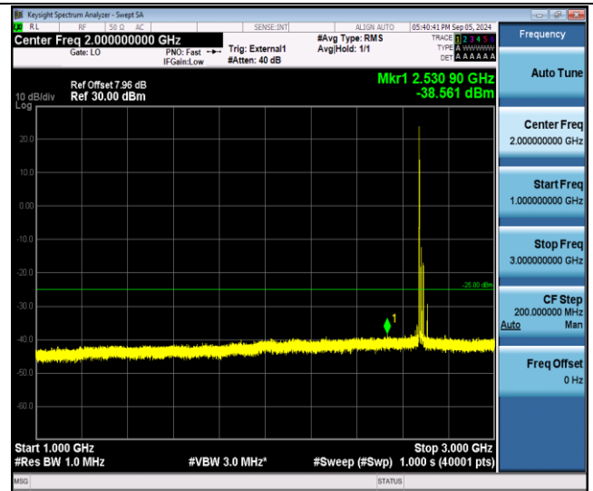
Band41-20MHz-QPSK-41490-1RB#0-1000~3000-PASS
