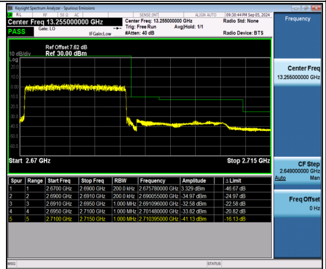
Band41-20MHz-QPSK-41490-100RB#0-PASS
