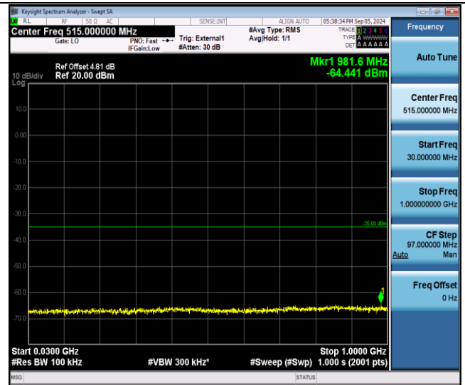
Band41-20MHz-QPSK-40620-1RB#0-30~1000-PASS
