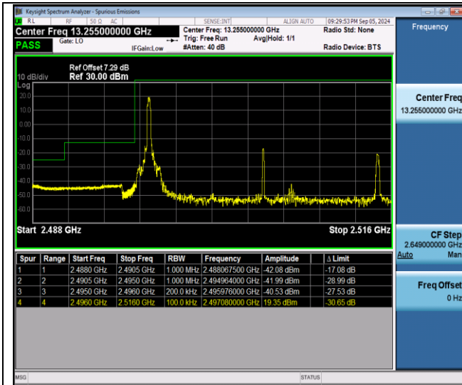
Band41-20MHz-QPSK-39750-1RB#0-PASS
