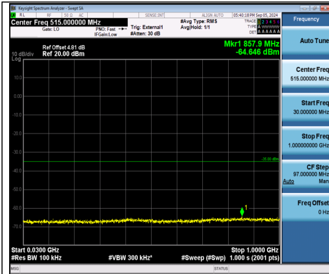
Band41-20MHz-QPSK-41490-1RB#0-30~1000-PASS
