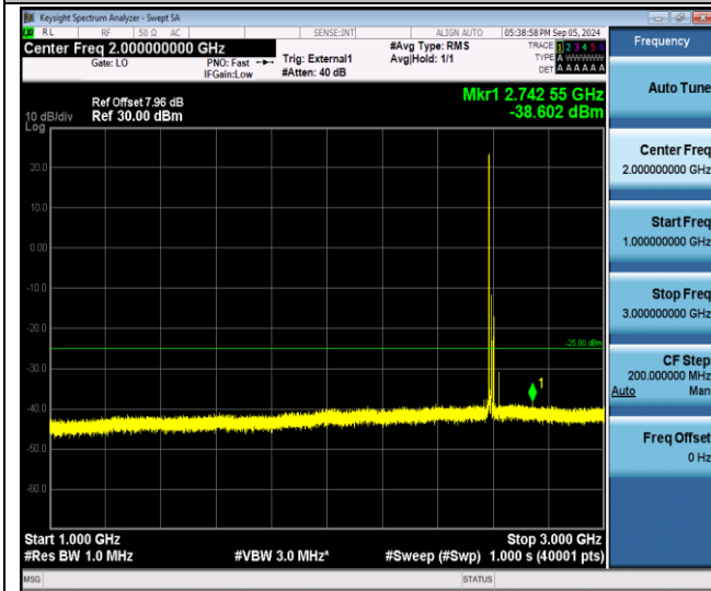
Band41-20MHz-QPSK-40620-1RB#0-1000~3000-PASS
