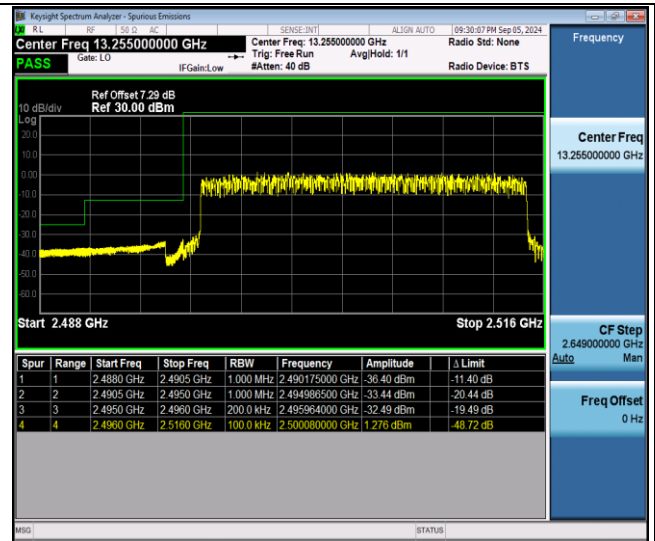
Band41-20MHz-QPSK-39750-100RB#0-PASS
