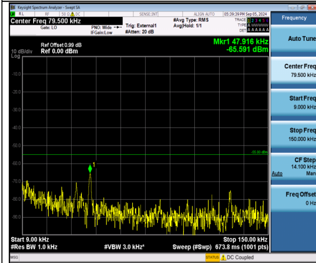
Band41-20MHz-QPSK-41490-1RB#0-0.009~0.15-PASS
