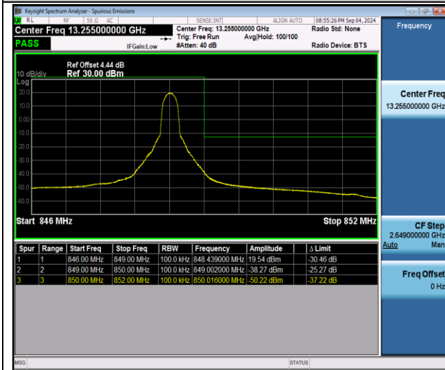
Band5-10MHz-QPSK-20600-1RB#49-PASS
