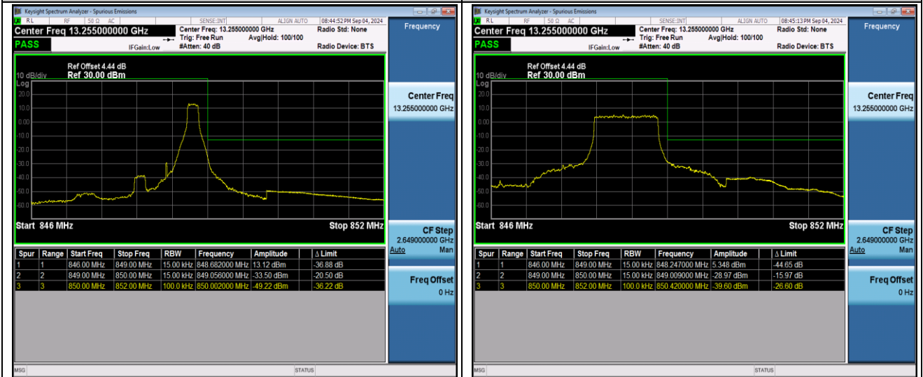
Band5-1.4MHz-QPSK-20643-1RB#5-PASS
