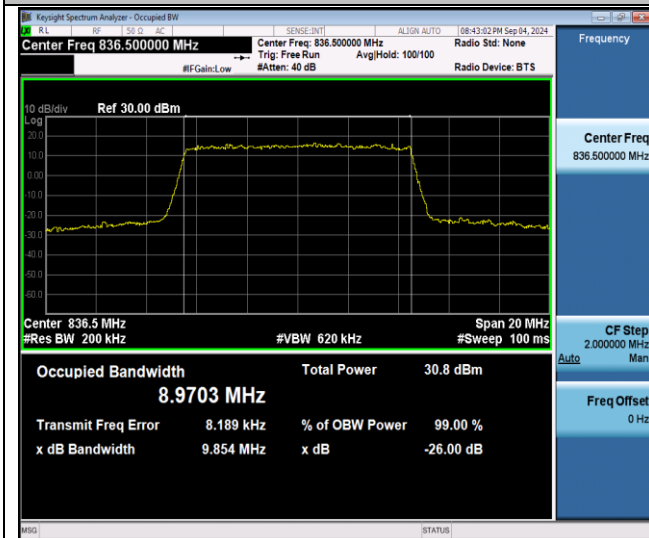
Band5-10MHz-16QAM-20525-50RB#0-PASS
