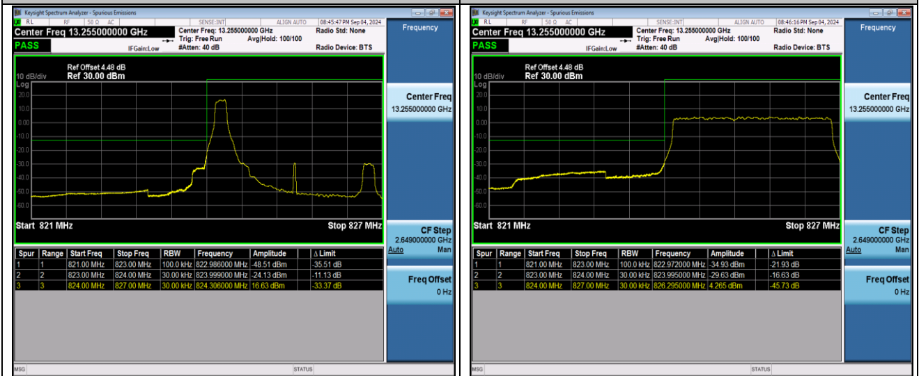
Band5-3MHz-QPSK-20415-1RB#0-PASS
