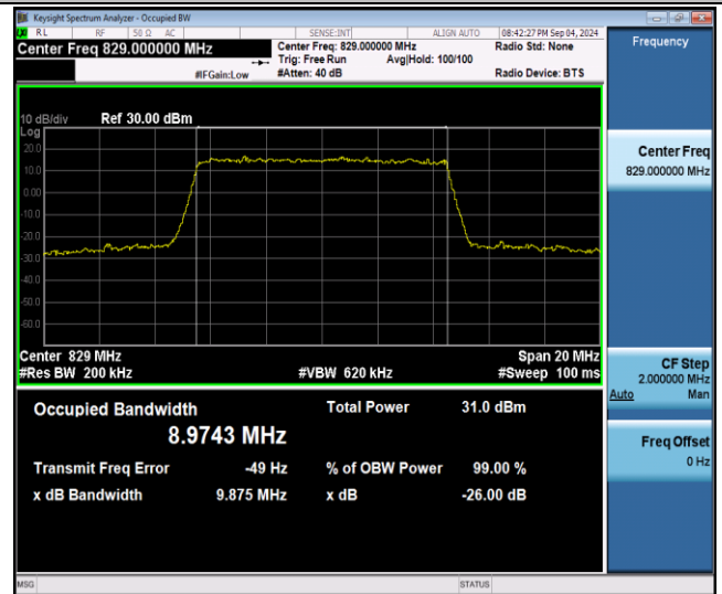
Band5-10MHz-16QAM-20450-50RB#0-PASS
