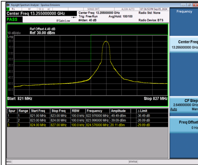
Band26(824-849)-10MHz-QPSK-26840-1RB#0-PASS
