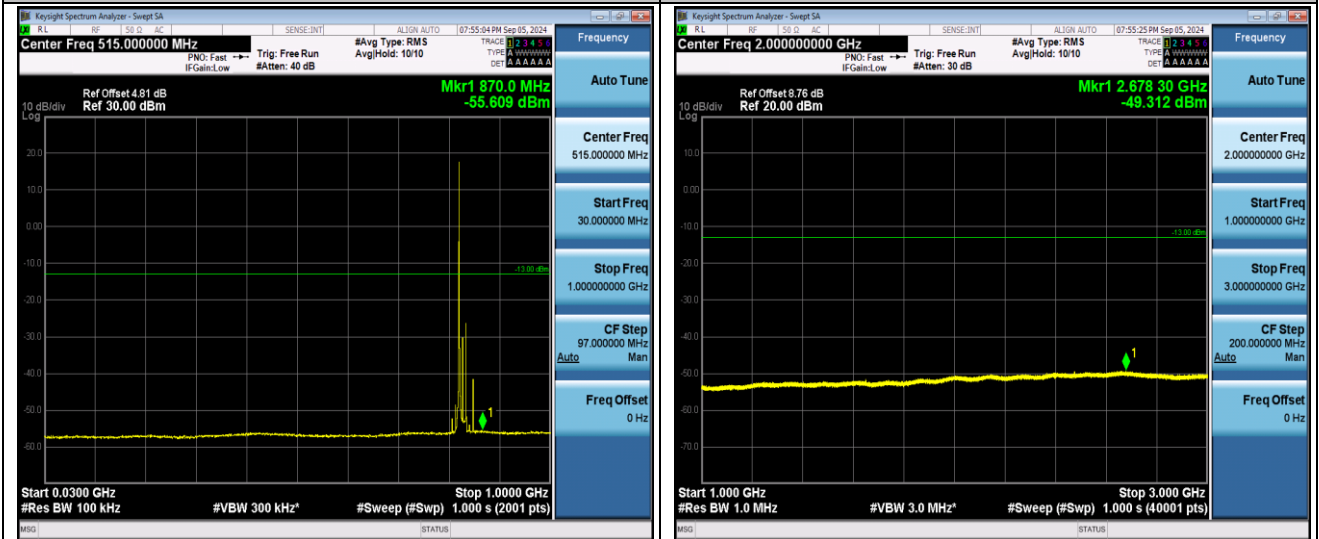
Band26(824-849)-15MHz-QPSK-26865-1RB#0-30~1000-PASS
