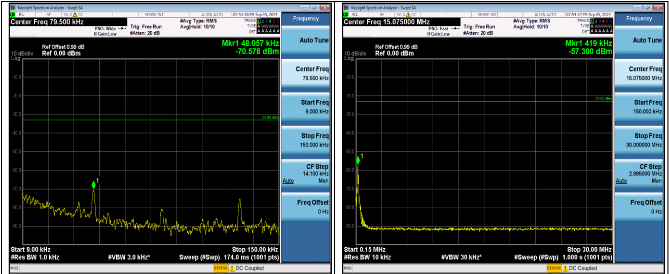
Band26(824-849)-15MHz-QPSK-26865-1RB#0-0.009~0.15-PASS
