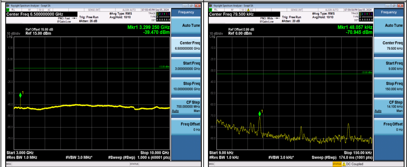
Band26(824-849)-15MHz-QPSK-26865-1RB#0-3000~10000-
