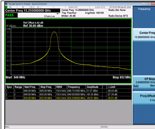
Band26(824-849)-15MHz-QPSK-26965-1RB#74-PASS
