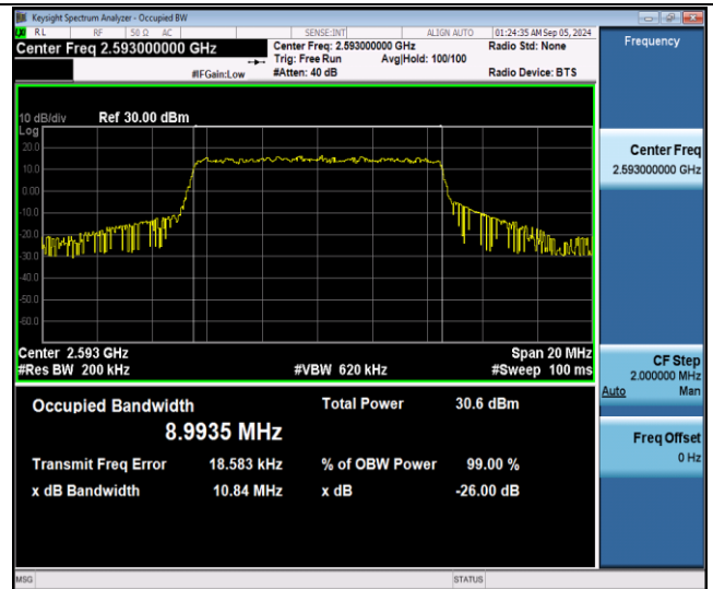
Band41-10MHz-QPSK-40620-50RB#0-PASS
