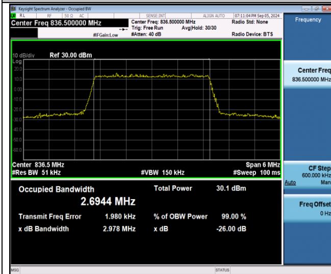
Band26(824-849)-3MHz-16QAM-26915-15RB#0-PASS
