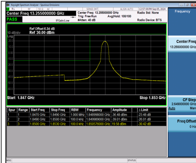
Band25-10MHz-QPSK-26090-1RB#0-PASS
