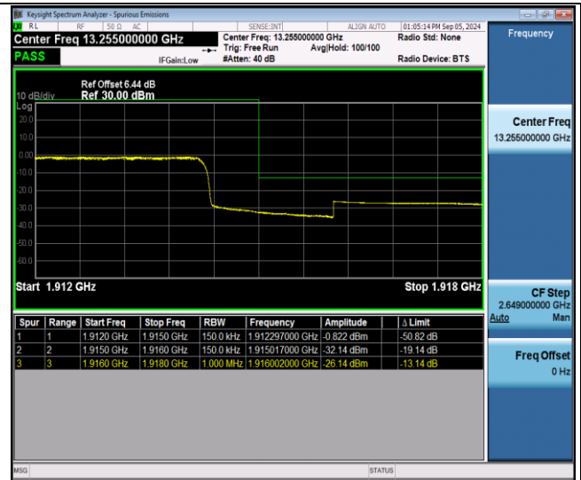
Band25-15MHz-QPSK-26615-75RB#0-PASS
