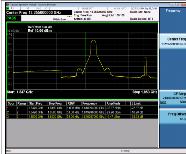
Band25-5MHz-QPSK-26065-1RB#0-PASS
