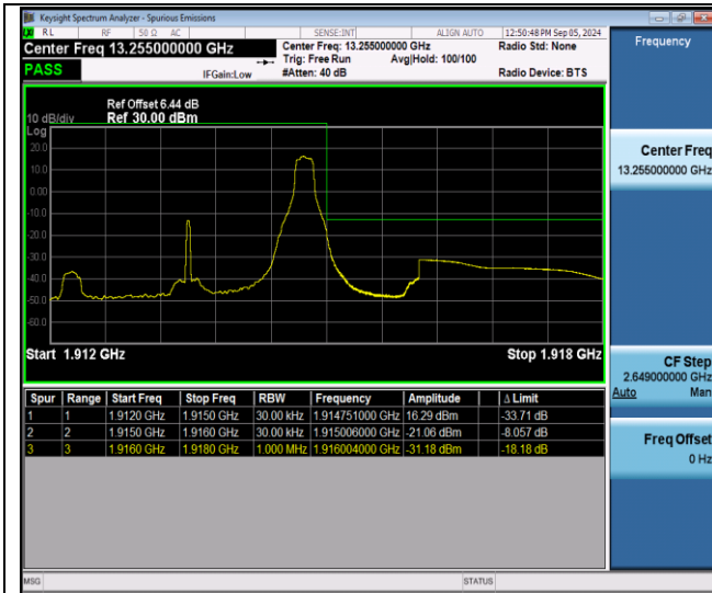
Band25-3MHz-QPSK-26675-1RB#14-PASS
