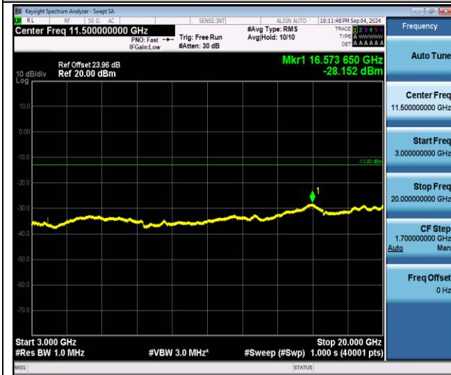
Band25-20MHz-QPSK-26590-1RB#0-3000~20000-PASS
