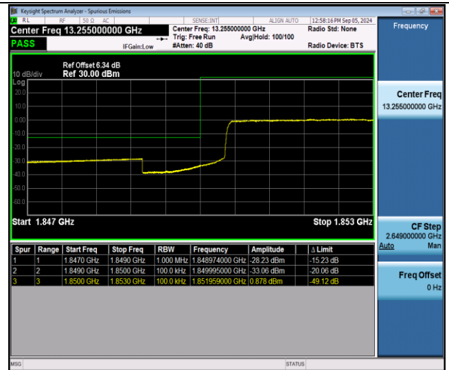
Band25-10MHz-QPSK-26090-50RB#0-PASS
