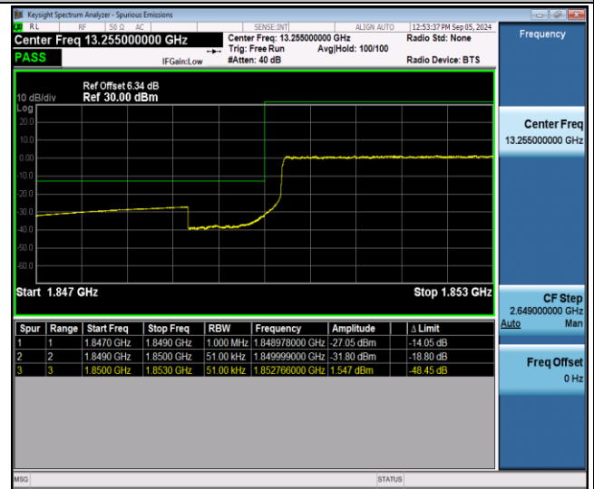
Band25-5MHz-QPSK-26065-25RB#0-PASS
