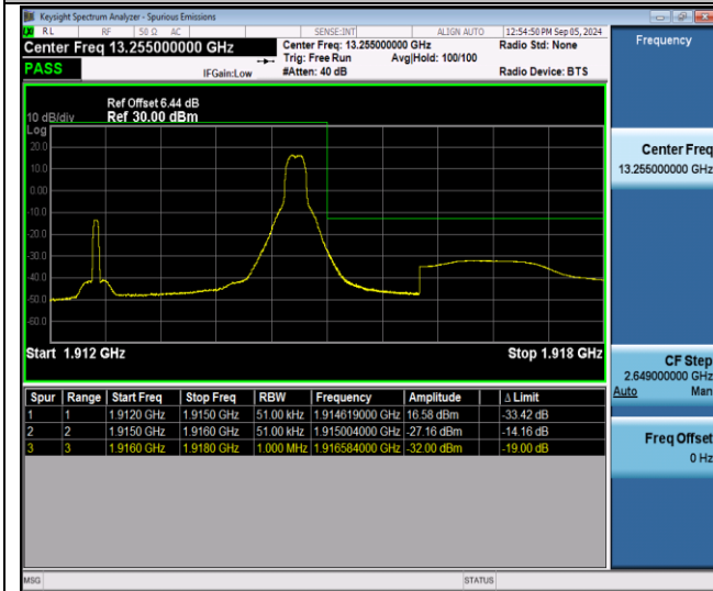
Band25-5MHz-QPSK-26665-1RB#24-PASS
