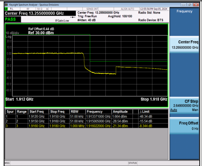
Band25-5MHz-QPSK-26665-25RB#0-PASS
